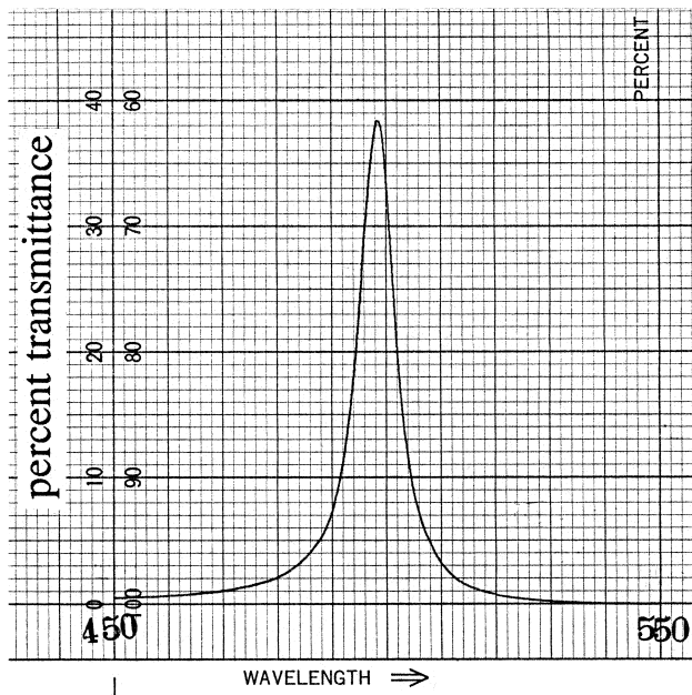
Fig. 1. Spectral transmittance of the BP-50 band pass filter.
