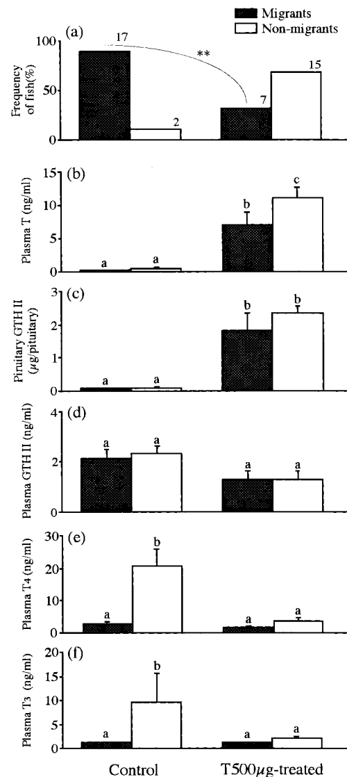
Fig. 1. Frequency of migrants and non-migrants, plasma levels of T, pituitary contents of GTH II, and plasma levels of GTH II, T_4 , and T_3 in controls and T500 \mu\text{g} -treated smolts. Figures beside columns indicate the number of migrants or non-migrants. Hormone levels are expressed as the mean and standard error. ** indicates significant difference at P < 0.01 . Differing letters represent significant differences at P < 0.05 among all groups.
