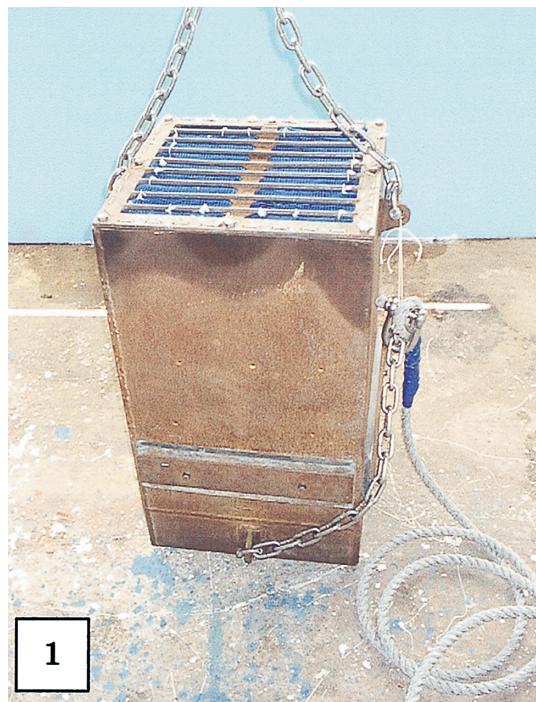
Fig. 1. Photograph of the dredger used in this study. In this photograph, the dredger is upside down. The dredger was suspended in this position temporarily at 5 m above the sea bottom. When the dredger stopped swinging, it was dropped down to the sea bottom in this upside-down position. The dredger stuck in the mud at the bottom. Then, the rope attached to the side of the dredger was pulled by a winch in order to rotate the dredger in the mud. The dredger with specimens was lifted from the mud in the upright position onto the research ship.
