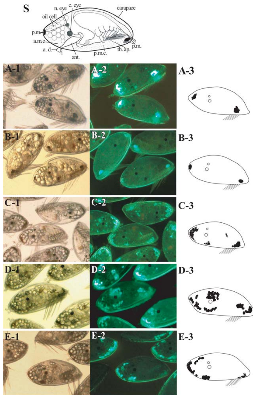
Fig. 1. Fluorescent patterns of balanomorph cyprids in group A. (S) A schematic of cyprid general features (After Walley, 1969; Anderson 1994). a.d., adhesive disk; ant., antennule; a.m.c., anterior mantle cavity; c. eye, compound eye; n. eye, nauplius eye; p.m., pigment mass; p.m.c., posterior mantle cavity; th. ap., thoracic appendages. (A) A. amphitrite , (B) A. improvisus , (C) A. eburneus , (D) A. reticulatus , (E) F. albicostatus . (A-1) – (E-1) are photographs under incident light, (A-2) – (E-2) are photographs under a fluorescent SZX-FBV filter unit. (A-3) – (E-3) are schematics of FPs. The fluorescent areas are black dots and black parts. Scale bar, 500 µm.
