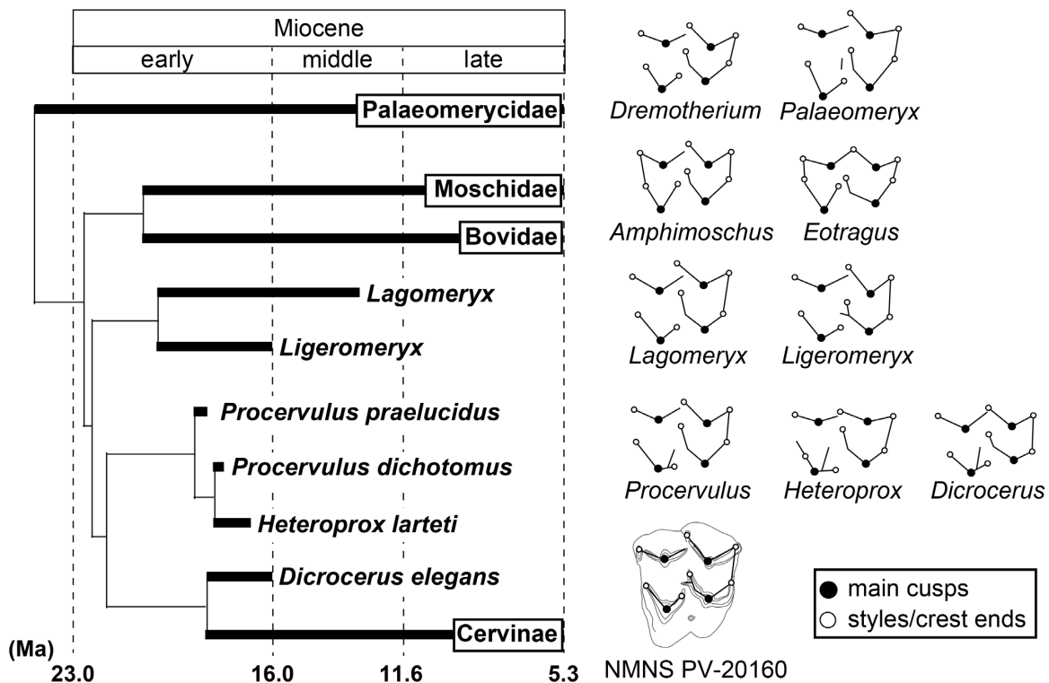
Figure 4. Comparisons of the left upper molar patterns commonly found in the examined pecoran specimens in Appendix 1. The phylogenetic tree was drawn by compiling the data of Suraprasit et al. (2014), S  nchez et al. (2015), and Mennecart et al. (2017).
