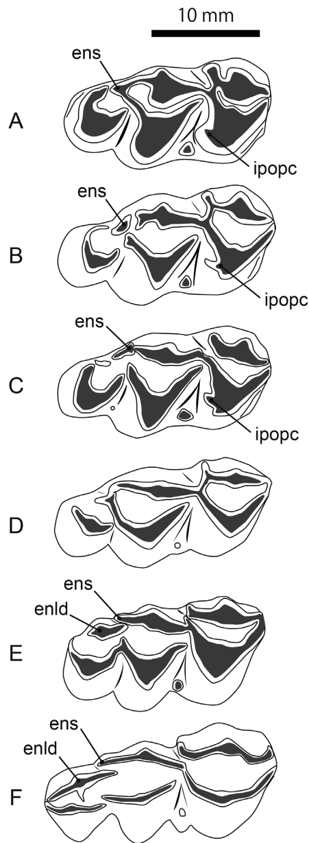
Figure 5. Comparisons of m3 of Miocene pecorans. A , Cervidae gen. et sp. indet. (NMNS PV-20161, mirror image); B , Ligeromeryx praestans (NMB S.O.2060, mirror image); C , Procervulus dichotomus (BSPG 1979XV555); D , Eotragus clavatus (NMB Ss.5789); E , Amphimoschus pontelevisensis (NMB S.O.72); F , Amphimoschus sp. (FPDM-V-8462). Abbreviations: ipopc, internal postprotocristid; enld, entoconulid; ens, entostylid.
