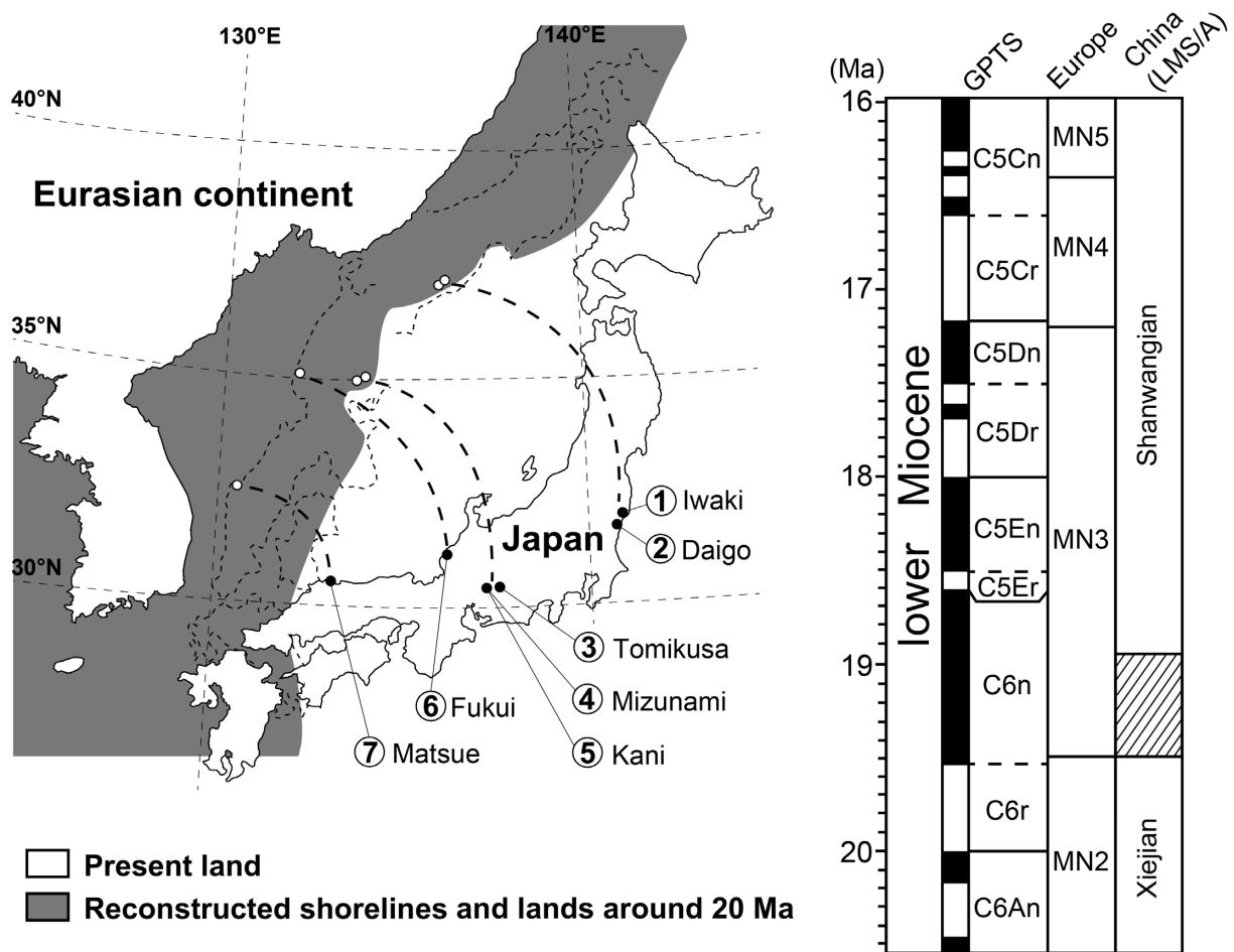
Figure 1. Fossil localities and chronostratigraphy of the lower Miocene pecorans (only body fossils) from Japan. A paleogeographic map of Japan and East Asia in 20 Ma was referred from Noda and Goto (2004). The locality numbers correspond to the numbers in Table 1. Geomagnetic polarity timescale (GPTS) follows Raffi et al. (2021). The biostratigraphic correlation of European MN zones and Chinese land mammal stage/age (LMS/A) follows Hilgen et al. (2012) and Qiu et al. (2013).
