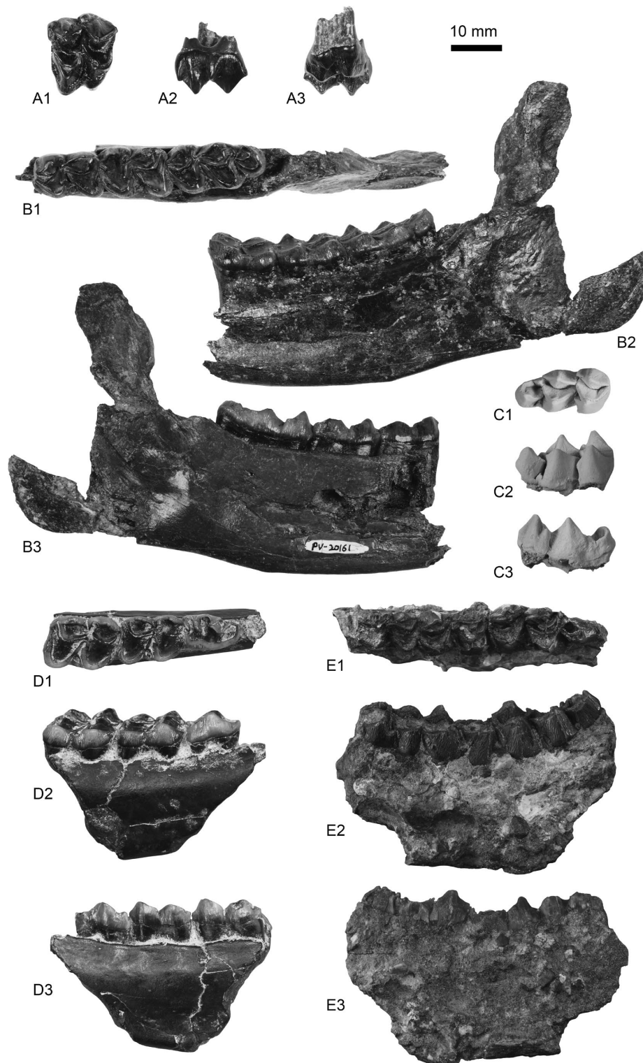
Figure 3. Cervidae gen. et sp. indet. (A–C) and Dicrocerus? tokunagai (D–E) from the lower Miocene of Japan. A , left M2 (NMNS PV-20160); A1, occlusal view; A2, labial view; A3, lingual view; B , a left mandible with m1–m3 (NMNS PV-20161); B1, occlusal view; B2, labial view; B3, lingual view; C , right m3 (MFM18126 in Nishioka and Ando, 2016); C1, occlusal view; C2, labial view; C3, lingual view; D , a right mandible with p4–m2 (NMJH A-636-1-1-9); D1, occlusal view; D2, labial view; D3, lingual view; E , a left mandible with m1–m3 (ICM YH-3412); E1, occlusal view; E2, labial view; E3, lingual view.
