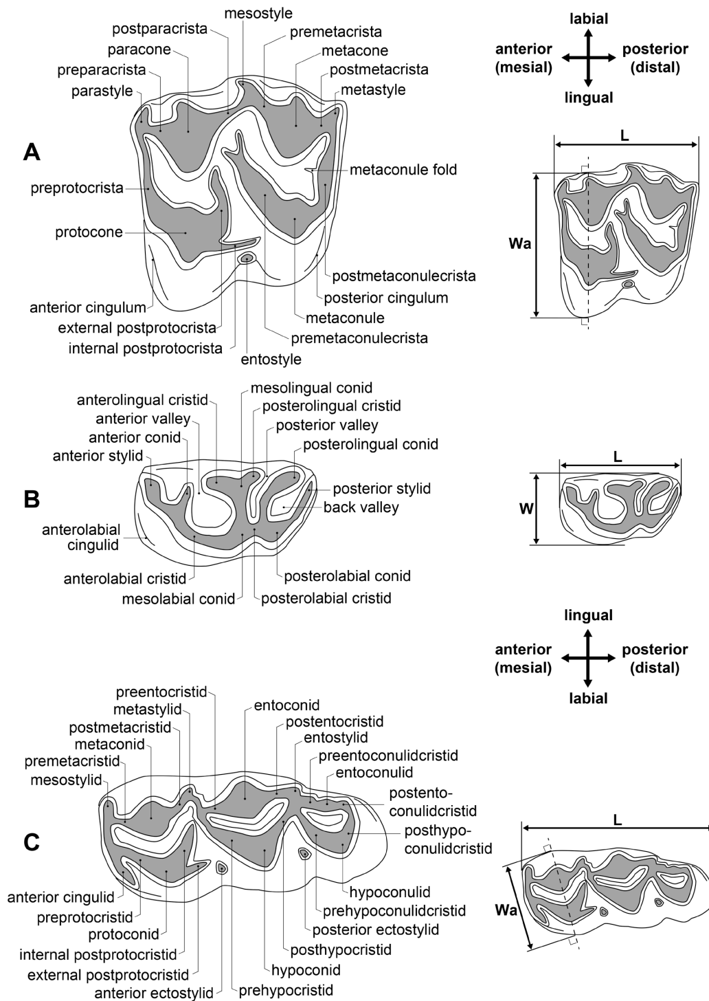
Figure 2. Dental terminology (after Bärmann and Rössner, 2011) and measuring points of left cheek teeth of pecorans. A , upper molar; B , lower premolar; C , lower molar.
