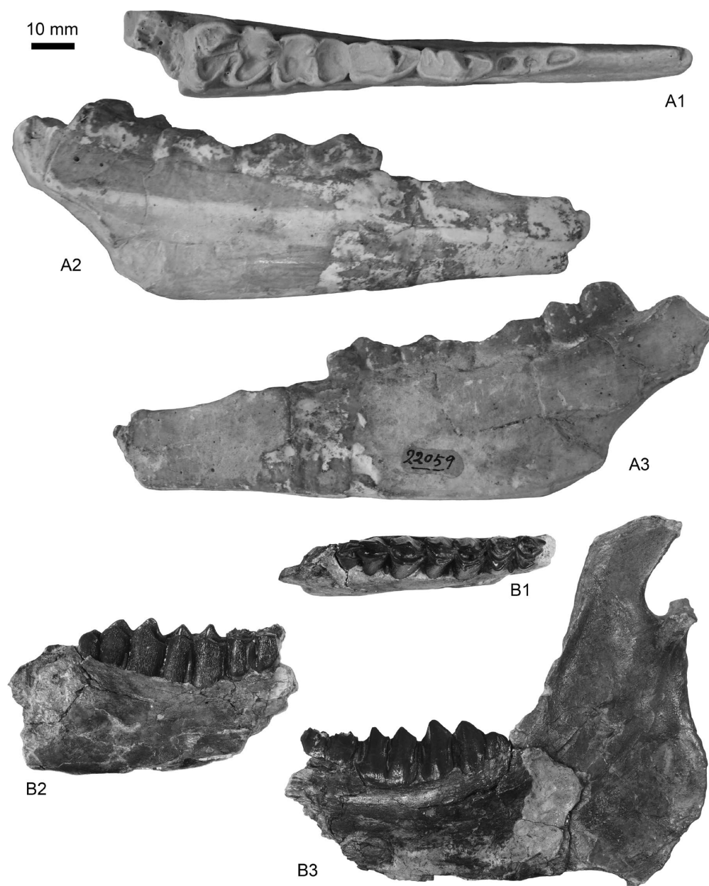
Figure 6. Cf. Palaeomeryx minoensis (A) and Amphimoschus sp. (B) from the lower Miocene of Japan. A , a right mandible with p3–m2 (IGPS 22059); A1, occlusal view (resin cast molded from IGPS 22059); A2, labial view (original cast); A3, lingual view (original cast); B , a right mandible with m1–m3 (FPDM-V-8462); B1, occlusal view; B2, labial view; B3, lingual view with the ramus.
