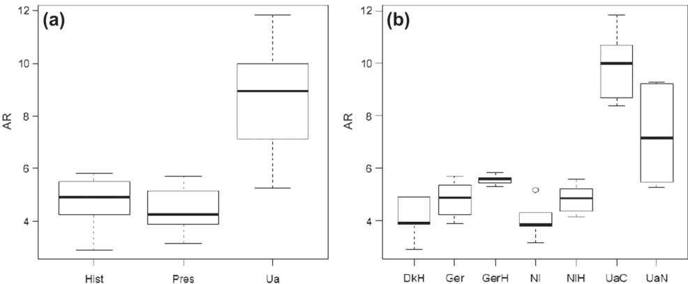
Figure 4. The differences in microsatellite allelic richness of European populations of black grouse: (a) the populations pooled in three categories – the present European (Pres), the historic European (Hist) and Ukrainian (Ua); (b) the populations considered as separate units: Danish historical (DkH), German present (Ger), German historical (GerH), Dutch present (NI), Dutch historical (NIH), Carpathian Ukrainian (UaC) and northern Ukrainian (UaN). Boxes represent median (thick line through boxes) and 75% (upper and lower end of boxes) and 95% (upper and lower hinges) interquartile ranges. Circles are outside values.
