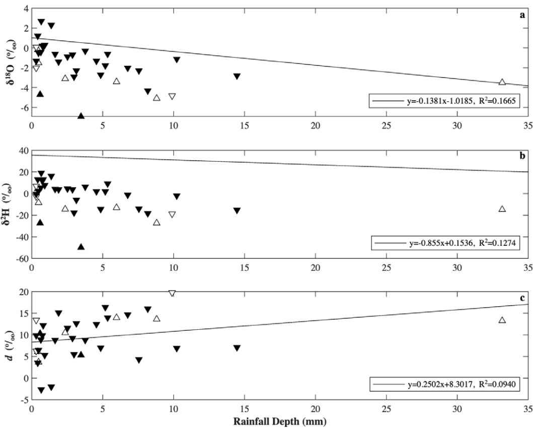
FIGURE 3. Linear regression of (A) \delta^{18}\text{O} , (B) \delta^2\text{H} , and (C) d values, from event-based precipitation, against corresponding rainfall depth. There is no relationship between rainfall depth and any of the stable isotope variables.
