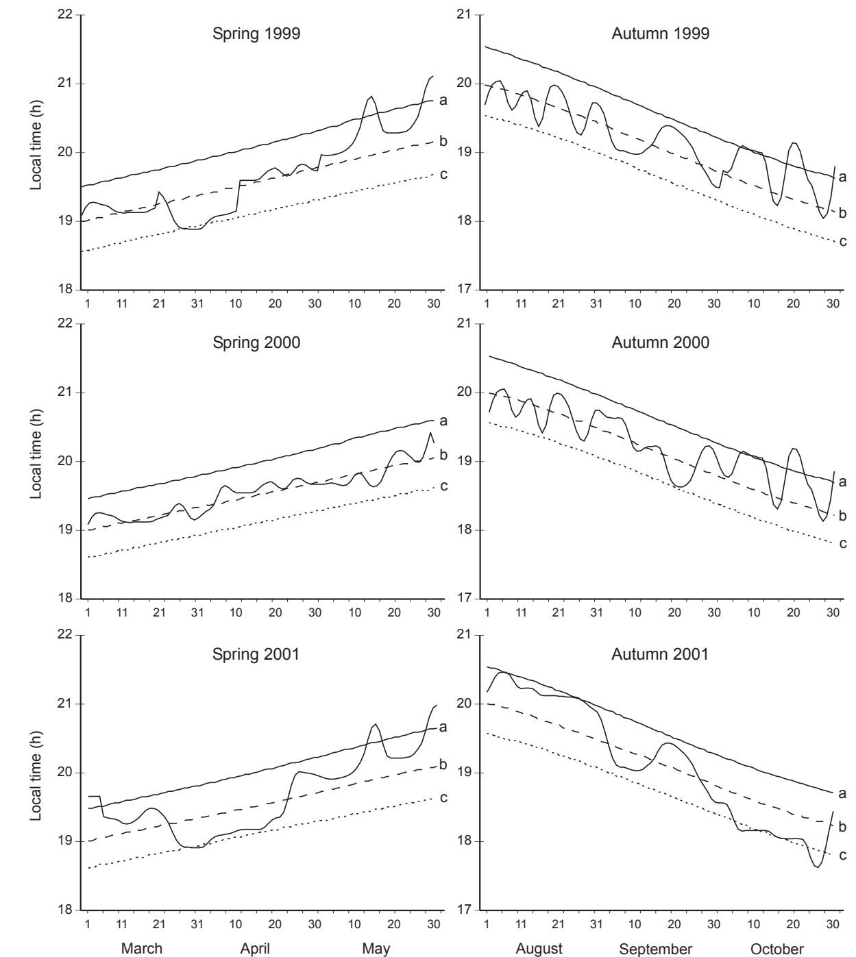
Fig. 1. Beginning of night migration (local time) related to the time of night (a), civil twilight (b) and sunset (c) in spring and autumn 1999–2001. Smoothed curve — sliding averages.
