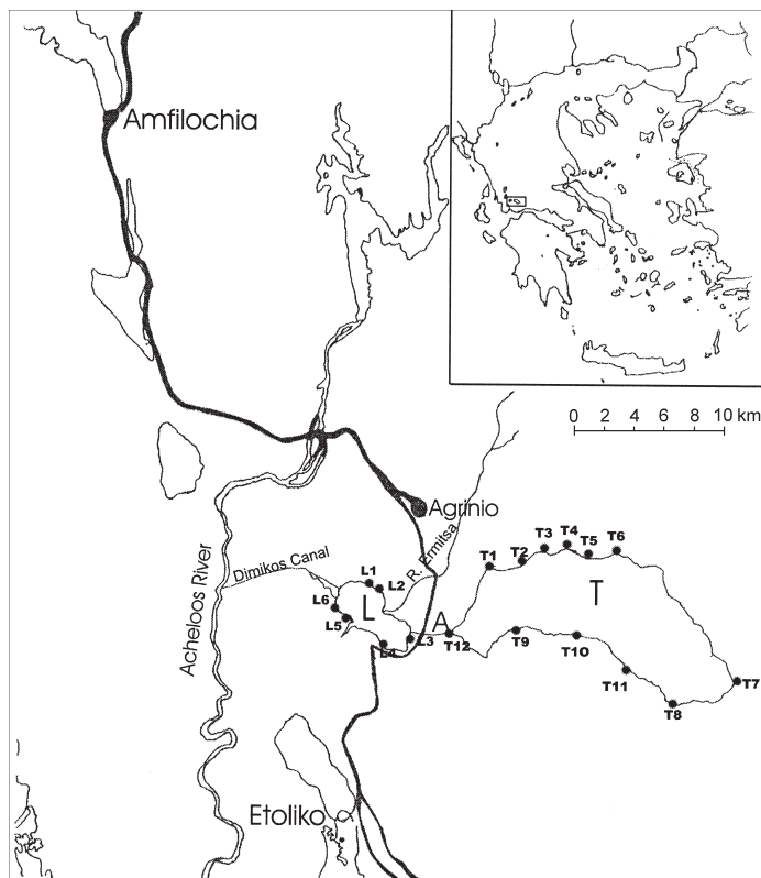
Fig. 1. Map of the lakes Trichonis (T) and Lisimachia (L), connected via the Alampei ditch (A), with the codes of the plant collection localities (see text).
