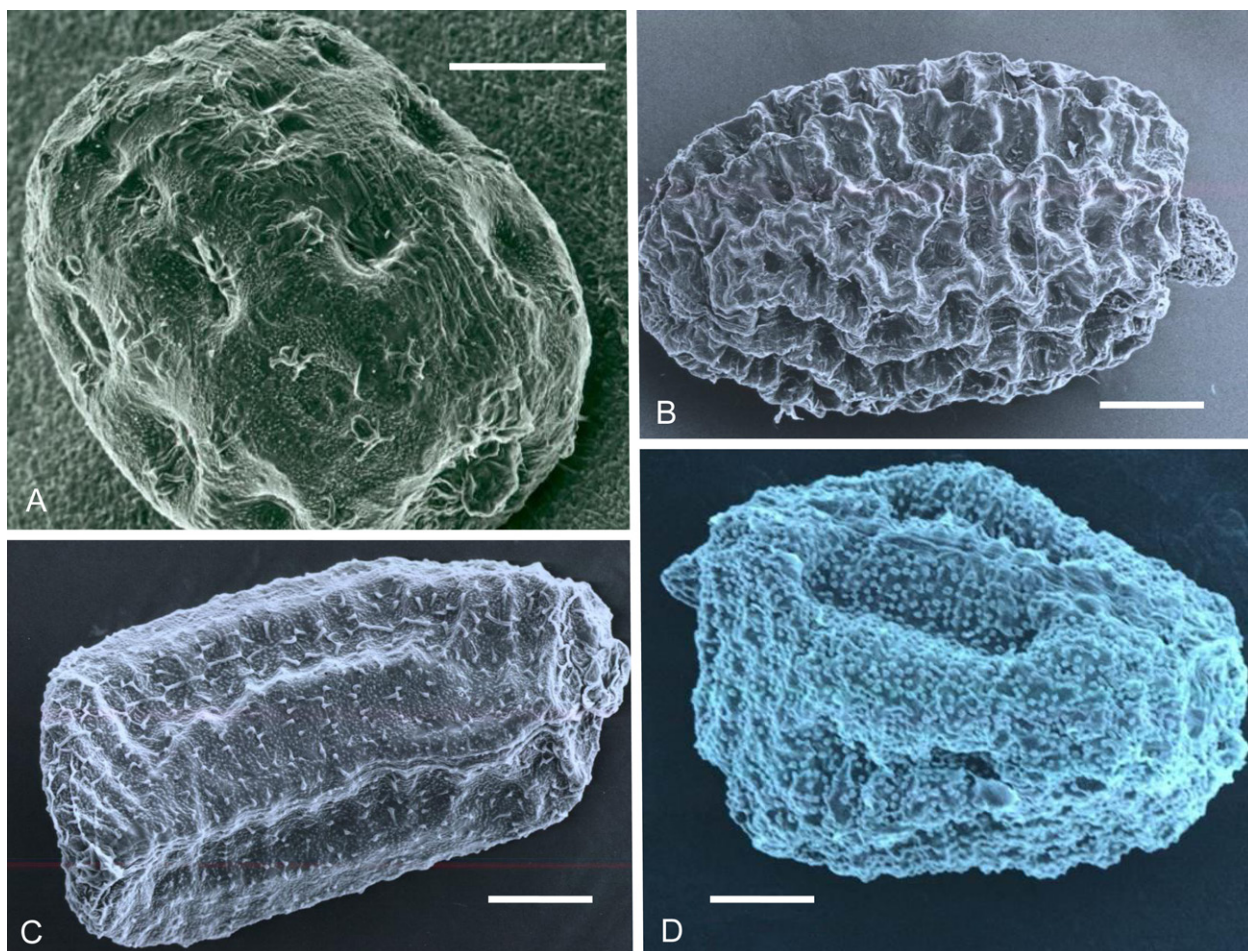
Fig. 3. SEM photographs of Linderniaceae seeds – A: Torenia crustacea ; B: Linderniella cerastioides ; C: Lindernia rotundifolia ; D: Crepidorhopalon microcarpaeoides . – Scale bar 100 µm. – Photographs by E. Fischer.
