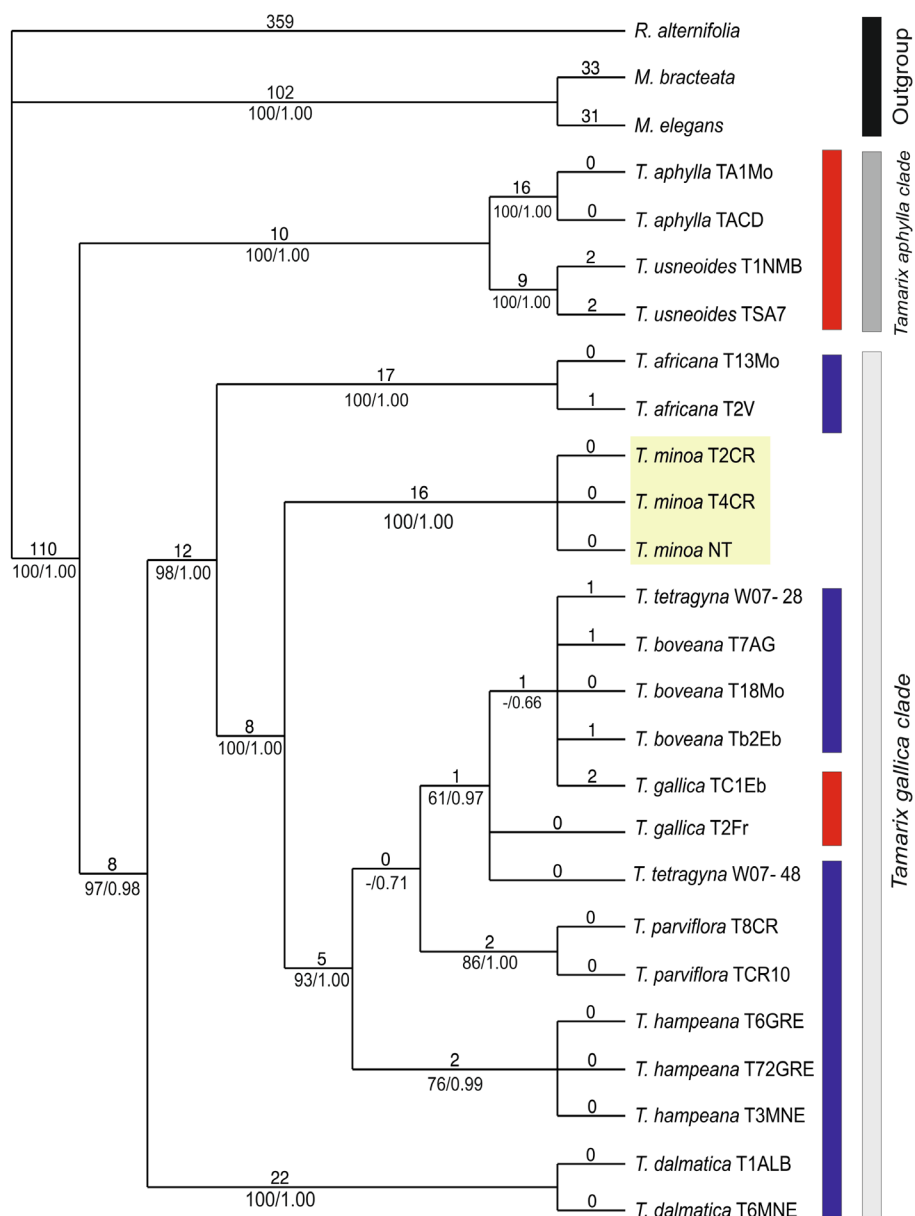
Fig. 3. One of the six most parsimonious trees obtained (774 steps, CI 0.935, RI 0.916). Branch lengths for parsimony analysis are shown above branches. Bootstrap values (BS) > 50% and Bayesian posterior probability (PP) > 0.90 are shown below branches (BS/PP). The outer vertical bars represent the outgroup and the two first split clades in Tamarix . The inner vertical bars represent the sections accepted by Baum (1978).
