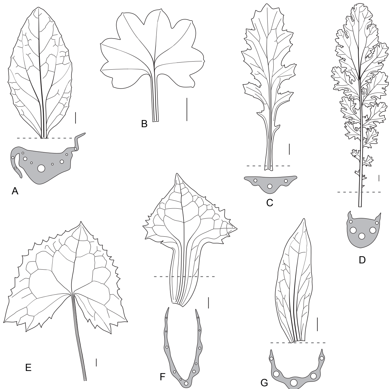
Fig. 1. Leaf shape and venation (abaxial leaf surface) and cross-sections (A, D, F, G; level of section indicated by dashed lines) of leaf bases. – A: Tephroseris integrifolia ; B: T. newcombei ; C: Senecio vulgaris ; D: Jacobaea vulgaris ; E–G: Ligularia stenocephala ; E: basal leaf; F: middle cauline leaf; G: upper cauline leaf. – Circles in cross-sections represent vascular bundles. – Scale bars: all 5 mm.
