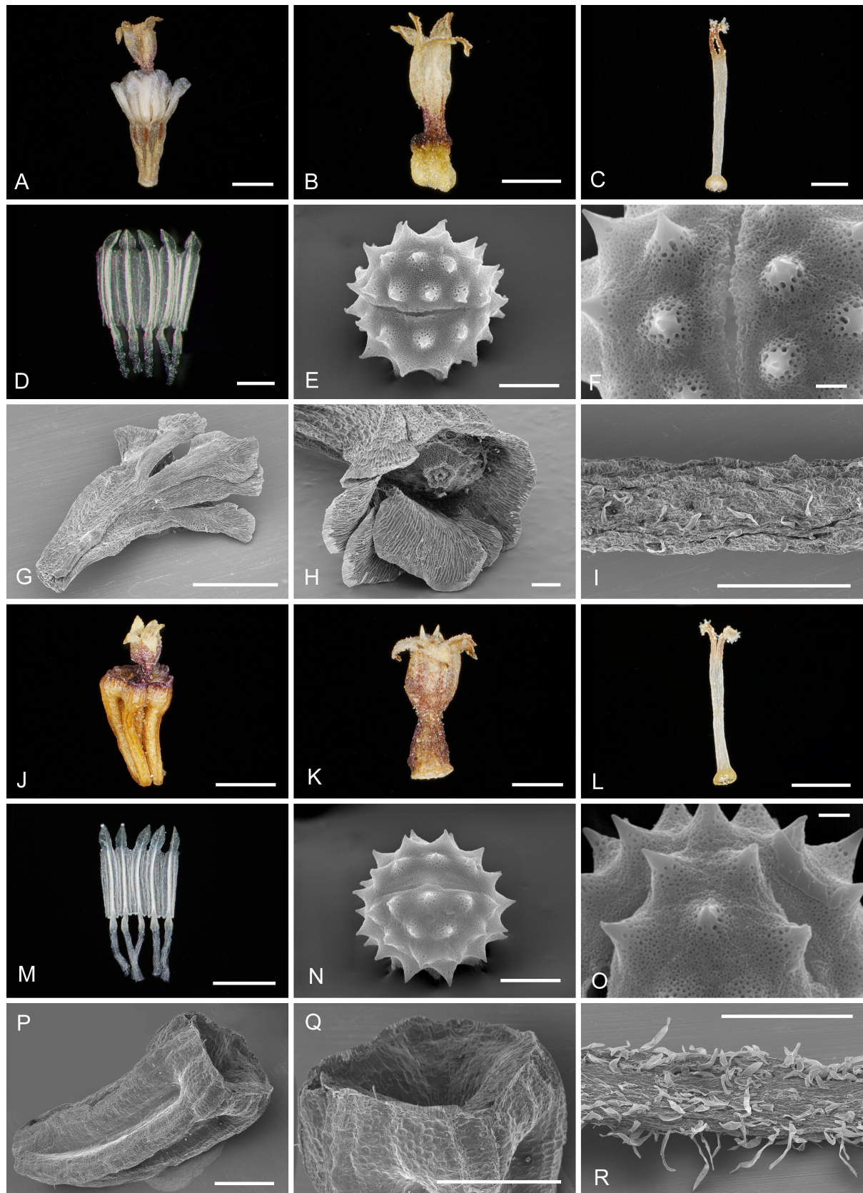
Fig. 2. Light microscope and SEM micrographs from A–I: Heteromera fuscata (Vogt 12847 & Oberprieler 7152) and J–R: H. philaenorum (Vogt 13007 & Oberprieler 7312). – A: disc floret; B: corolla of disc floret; C: style; D: stamens; E: pollen grain; F: detail of pollen grain; G: achene; H: apical part of achene; I: hairs on leaf; J: disc floret; K: corolla of disc floret; L: style; M: stamens; N: pollen grain; O: detail of pollen grain; P: achene; Q: apical part of achene; R: hairs on leaf. – Scale bars: A, B, G, I, K–M, P–R = 1 mm; C, D = 500 \mu m; E, N = 10 \mu m; F, O = 2 \mu m; H = 200 \mu m.
