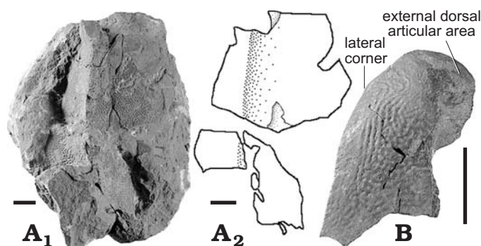
Fig. 8. Dermal plates of antiarch placoderm Asterolepis sp. 2., from Mazy (Namur Province), Givetian, Devonian. A. IRSNB P.9260, unassigned plate, external view; photograph ( A 1 ), explanatory drawing ( A 2 ). B. IRSNB P.9259, CD1, external view. Scale bars 10 mm.
