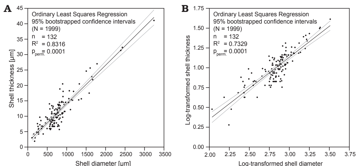
Fig. 3. Correlation between the shell thickness and shell diameter; by linear bivariate modelling using Ordinary Least Squares Regression in PAST3 (Hammer et al. 2001). A. The data show that the shell of Coelodiscus minutus is generally very thin and shows a linear increase with shell diameter; this linear increase is generally typical of shelled molluscs and is also present in modern holoplanktonic gastropods. B. The log-transformed data of the original measurements confirm the linear increase with shell diameter. Abbreviations: N, number of bootstrap replicates; n, number of measured specimens; R 2 , coefficient of correlation; p perm. , permutation test on correlation (R 2 ), using 9999 replicates.
