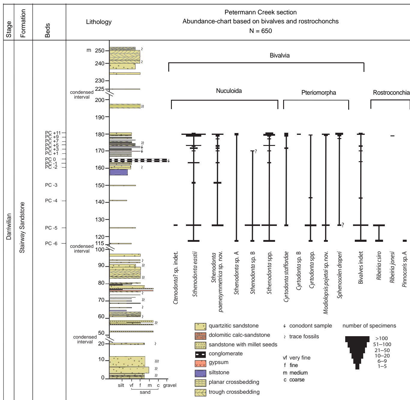
Fig. 5. Composite log of the Stairway Sandstone and abundance-charts showing distribution of bivalves and rostroconchs in the Petermann Creek section.
