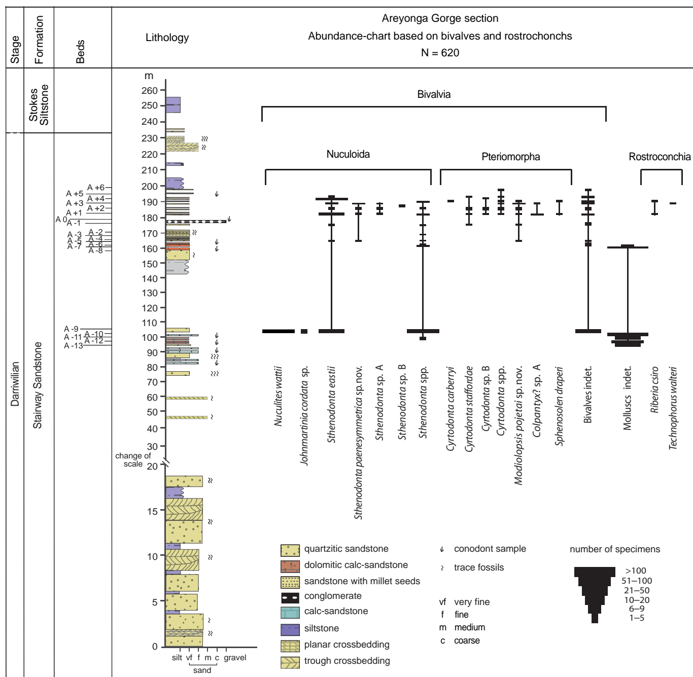
Fig. 4. Composite log of the Stairway Sandstone and abundance-charts showing distribution of bivalves and rostroconchs in the Areyonga Gorge section.
