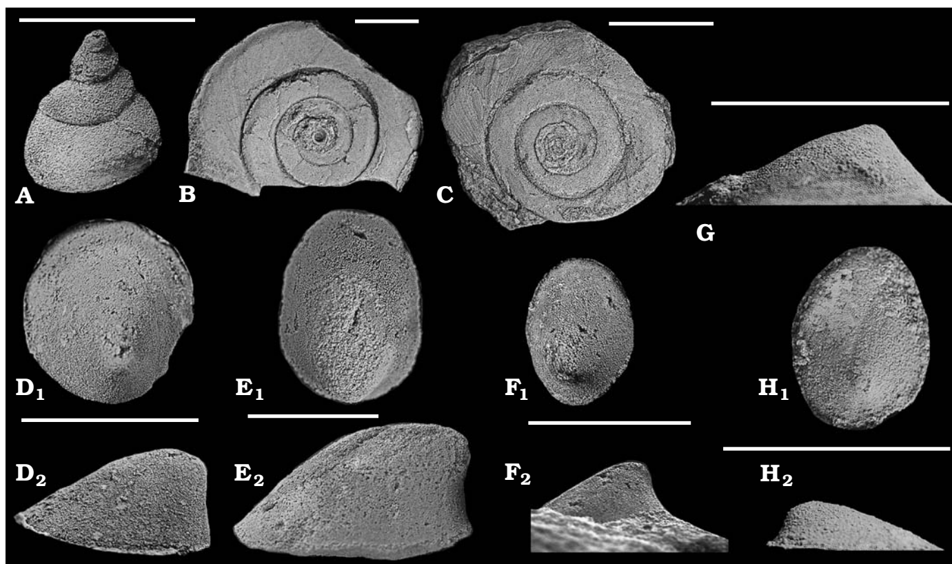
Fig. 13. Gastropods from the Stairway Sandstone, Middle Ordovician, Australia. All internal moulds. A. Raphistomina ? sp. from Areyonga Gorge with 4 whorls (CPC 41496). B, C. Teiichispira ? sp. from loose samples from Petermann Creek; with a very flat base, perhaps 5 whorls present ( B , CPC 41497; C , CPC 41498). D, E. Archinacelloid sp. A ( D , CPC 41499; E , CPC 41500) from Petermann Creek; with slightly concave subapical surface and steeply inclined slightly curved apex, in anterior ( D 1 , E 1 ) and left-lateral ( D 2 , E 2 ) views. F, G. Archinacelloid sp. B from Areyonga Gorge ( F ) and Petermann Creek ( G ). F. Specimen with subcentral and sharply pointed apex (CPC 41501), in anterior ( F 1 ) and left-lateral ( F 2 ) views. G. Specimen with subcentral and pointy apex (CPC 41502), in left-lateral view. H. Archinacelloid sp. C from Petermann Creek with low shell profile and inclined slightly curved apex (CPC 41503), in anterior ( H 1 ) and left-lateral ( H 2 ) views. Scale bar 10 mm.
