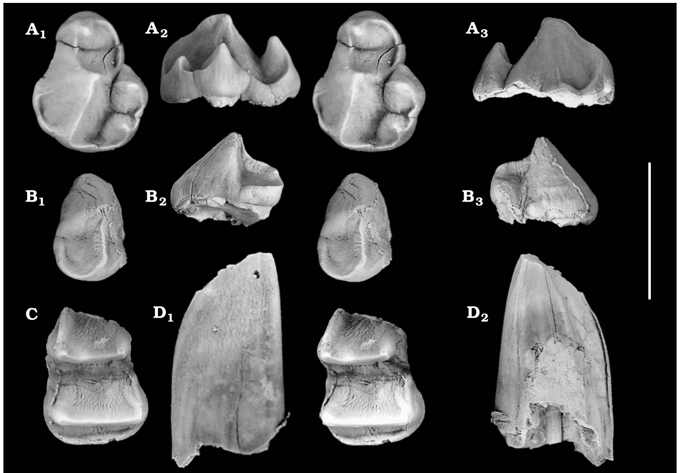
Fig. 4. Diprotodontid marsupial Neohelos davidrideri sp. nov. referred material from the Middle Miocene Jaw Junction LF, Riversleigh World Heritage Area, Queensland, Australia. A. QM F40178, RP3; occlusal stereopair (A 1 ), lingual (A 2 ), and buccal (A 3 ) views. B. QM F40182, Rp3; occlusal stereopair (B 1 ), lingual (B 2 ), and buccal (B 3 ) views. C. QM F40174, Lm1; occlusal stereopair. D. QM F40177, Li1; lingual (D 1 ) and buccal (D 2 ) views. Scale bar 20 mm.
