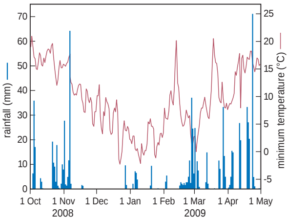
Figure 3. Daily precipitation (bars) and minimum temperatures (line) measured at Yueyang City (near to Caisang Lake) during winter 2008/2009.
