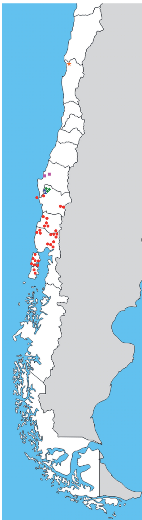
Fig. 83. Distribution map. (● red circles) Achilia excisa . (▲ blue triangles) A. pachycera . (◆ green diamonds) A. fiura . (■ pink squares) A. auriculata . (★ yellow stars) A. ovalensis .
