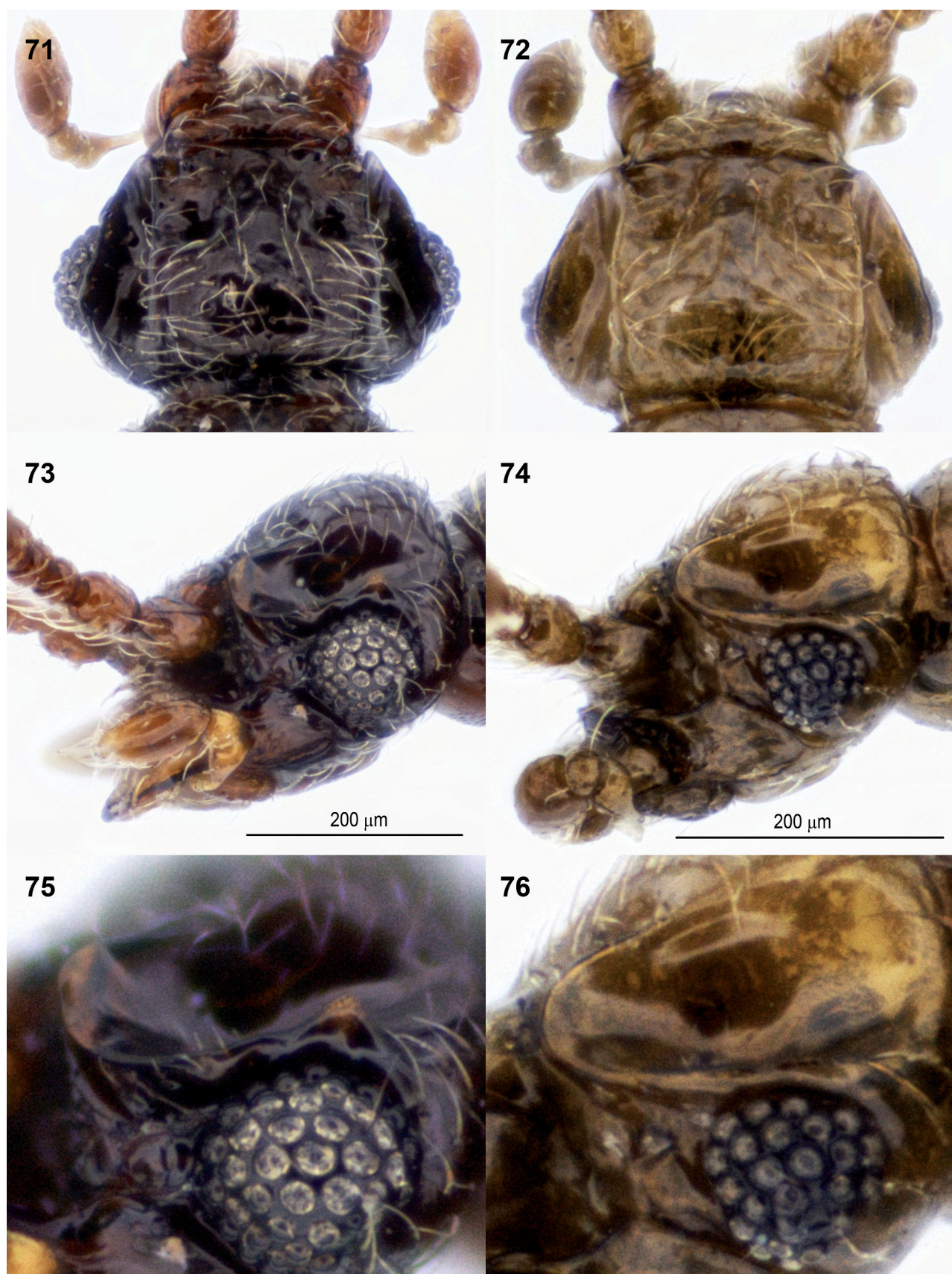
Figs 71-76. Achilia frontalis . (71, 73, 75) specimen from Chillán. (72, 74, 76) specimen from Frutillar. Male heads in dorsal (71-72) and lateral (73-74) views. (75-76) male supraocular area in lateral view. Scale bar left for (71, 73) and right for (72, 74).
