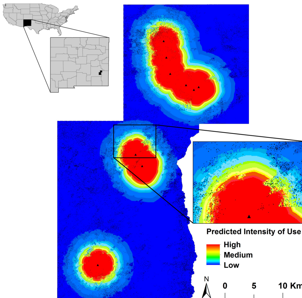
Figure 3. Predicted intensity of use of lesser prairie-chickens throughout their annual cycle in southeastern New Mexico is heavily influenced by mesquite distribution (inset; black dots) and centered around lek sites (closed triangles).
