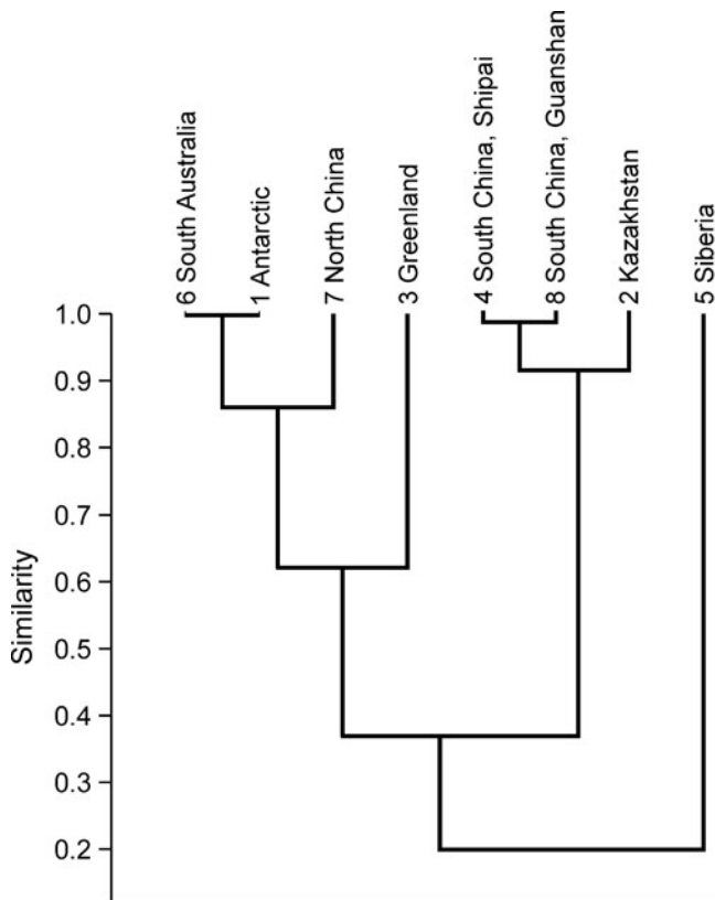
Figure 19. Results of the pair-group cluster analysis for the Cambrian Stage 4 linguliform genera from 8 localities (Raup-Crick similarity).
