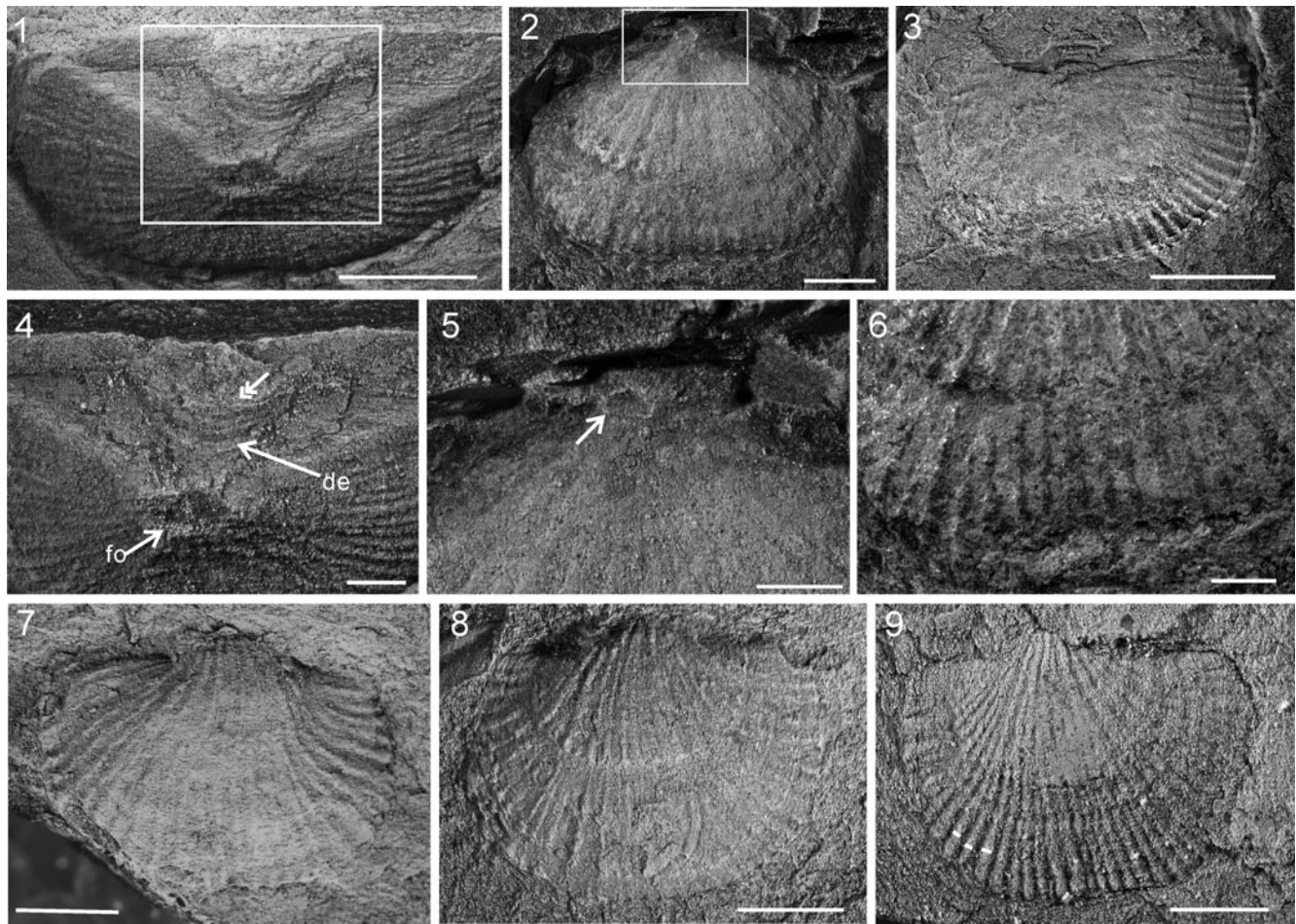
Figure 12. Nisusia liantuoensis from the lower Cambrian Shipai Formation at Xiachazhuang section. (1) Posterior view of ventral valve (ELI QJP-SP-015); (2, 3) ventral valves (ELI QJP-SP-045, ELI QJP-SP-006); (4) close-up view of (1) showing the apical foramen (fo, marked by arrow), developed pseudointerarea, deltidium (de, marked by arrow), and posterior median opening (marked by double arrows); (5) an enlargement of (2), showing the pedicle foramen (marked by arrow); (6) a fragment of one ventral valve, showing the radial lines on the shell surface (ELI QJP-SP-045); (7–9) dorsal valves (ELI QJP-SP-037, ELI QJP-SP-013, ELI QJP-SP-008). Scale bars = 3 mm (1, 7–9), 2 mm (2), 4 mm (3), or 1 mm (4–6).
