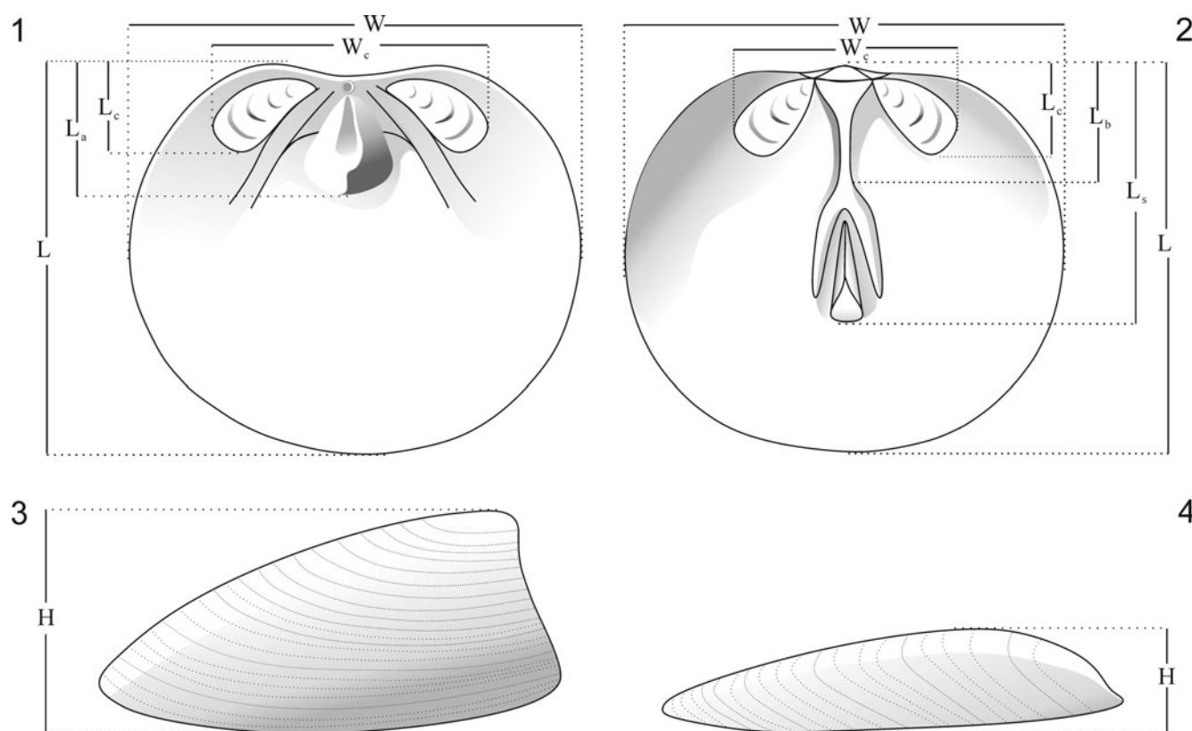
Figure 5. Schematic reconstruction of Linnarssonella sapushanensis from lower Cambrian Shipai Formation, showing location of measurements in Table 1. (1) Ventral interior; (2) dorsal interior; (3) lateral view of ventral valve; (4) lateral view of dorsal valve.
