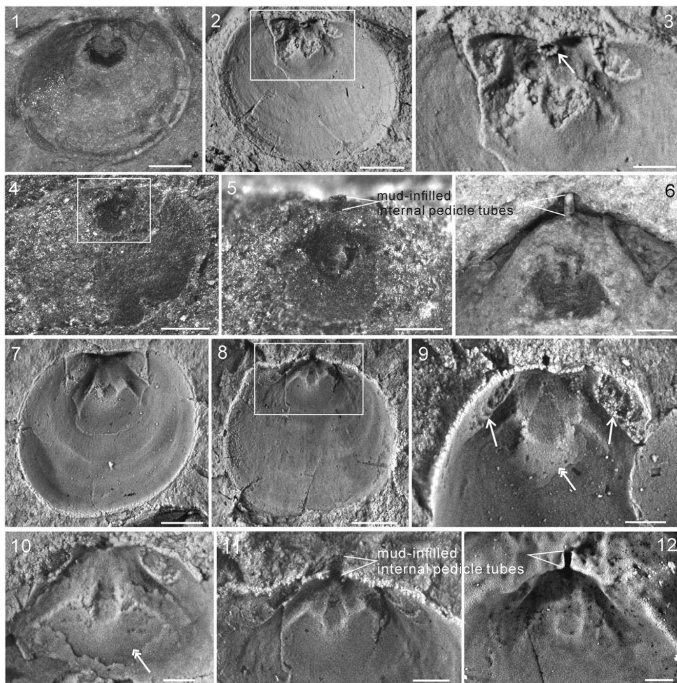
Figure 3. Ventral valves and latex casts of Linnarssonina sapushanensis from the lower Cambrian Shipai Formation at Xiachazhuang section, and comparison to L. sapushanensis from the Wulongqing Formation (Guanshan fauna). (1) Internal mold (ELI QJP-SP-357-2); (2) latex cast of (1); (3) an enlargement of (2), showing the pedicle opening (marked by arrow); (4) internal mold (ELI QJP-SP-040); (5) close-up view of (4), note the mud-infilled internal pedicle tube; (6) one specimen of L. sapushanensis with the mud-infilled pedicle tube from the Wulongqing Formation, eastern Yunnan (ELI CLP-007-12); (7, 8) latex casts (ELI QJP-SP-357-30, ELI QJP-SP-357-30); (9) latex cast showing cardinal muscle scars (marked by arrows) and apical process with a median groove (marked by double arrows) (ELI QJP-SP-357-37); (10) latex cast showing apical process with a median groove (marked by double arrows) (ELI QJP-SP-357-9); (11) an enlargement of (8), note the latex cast of mud-infilled internal pedicle tube; (12) latex cast of L. sapushanensis from the Wulongqing Formation, eastern Yunnan (ELI CLP-183-30). Scale bars = 500 \mu m (1, 2, 4, 7, 8), or 200 \mu m (3, 5, 6, 9–12).
