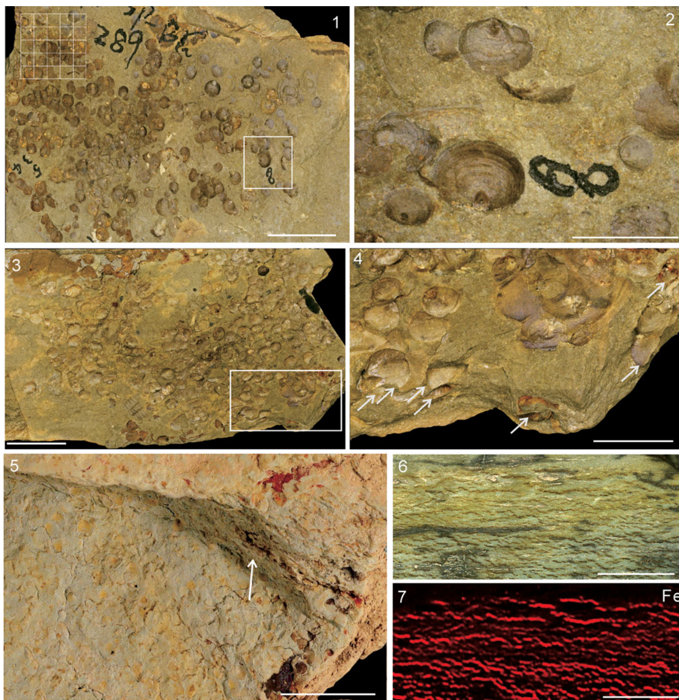
Figure 15. Acrotretoid brachiopod shell concentrations of Linnarssonina sapushanensis from the lower Cambrian Shipai Formation at Xiachazhuang section of Hubei Province, and comparison to shell beds of L. sapushanensis from the Wulongqing Formation of Yunnan Province. (1–4) Acrotretoid shell concentrations from the Shipai Formation: (1) shell valves aggregated as high-density concentrations on the bedding plane (ELI QJP-SP-289), with inset box indicating the position of (2) and grid in upper left used to count the number of shells in 1 cm 2 ; (2) close-up view of (1) showing acrotretoid shell valves of different sizes distributed on the bedding plane; (3) acrotretoid shell bed (ELI QJP-SP-357); (4) close-up view of (3) marked by an inset box, showing the acrotretoid shell valves distributed at different micro-layers of bedding planes (marked by white arrows); (5) multi-layered, high-density shell beds from Wulongqing Formation packed up to 2 cm thick (ELI SJJ-164); (6) longitudinally polished section of (5), showing frequent occurrences of the acrotretoid shell valves, aggregated approximately as 11–13 pavements within 1 cm thick muddy sediment; (7) micro-XRF mapping of (6), showing the rich content of Fe within the acrotretoids. Scale bars = 1 cm (1, 3, 5–7), 3 mm (2), 4 mm (4).
