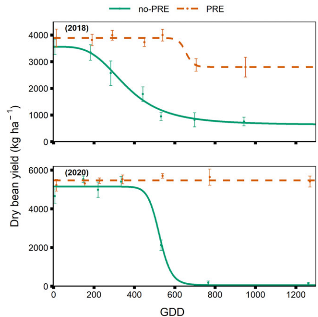
Figure 3. Dry bean yield in kg ha -1 in response to increasing duration of weed competition, presented by the number of growing degree days (GDD) accumulated after dry bean emergence, base 10C, for no-preemergence (no-PRE) and preemergence (PRE) treatments in 2018 and 2020.
