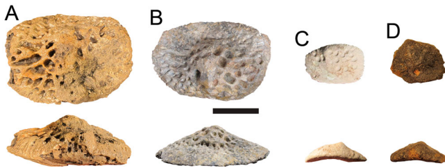
FIGURE 26. Comparison of dorsal osteoderms in dorsal and anterior views. A , Deinosuchus hatcheri , CM 963. B , Deinosuchus riograndensis , TMM 43620-1. C , Deinosuchus schwimmeri , ALMNH 1002. D , Deinosuchus schwimmeri , MMNS VP-5997. Scale bar equals 5 cm.
