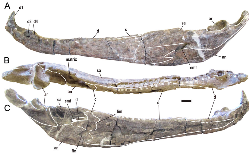
FIGURE 16. Deinosuchus riograndensis (TMM 43620-1) left hemimandible. A , lateral view. B , dorsal view. C , medial view. Abbreviations: an, angular; ar, articular; c, coronoid; d, dentary; d1, d3, d4, dentary teeth 1, 3, and 4; emf, external mandibular fenestra; fic, foramen intermandibularis caudalis; fim, foramen intermandibularis medius; s, splenial; sa, surangular. Scale bar equals 5 cm.
