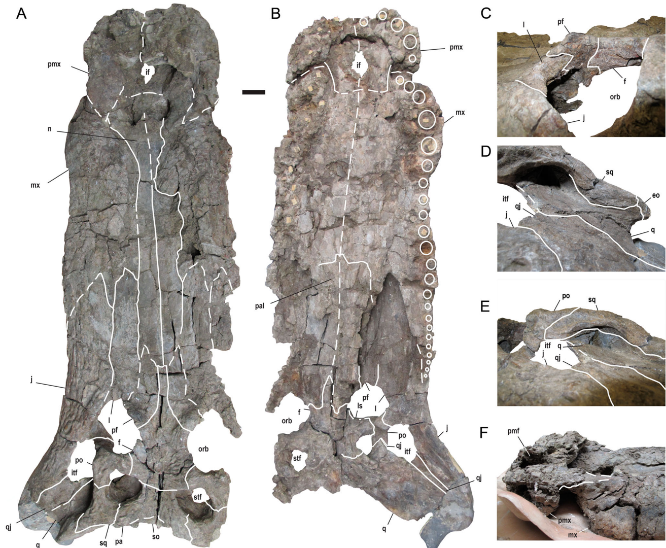
FIGURE 12. Deinosuchus riograndensis (TMM 43620-1) skull with elements illustrated. A , skull in dorsal view. B , skull in ventral view. C , left orbit in lateral view. D , left posterior-most skull in lateral view. E , left otic region in lateral view. F , left anterior-most snout in lateral view. Abbreviations: eo, exoccipital; f, frontal; if, incisive foramen; itf, infratemporal fenestra; j, jugal; l, lacrimal; ls, laterosphenoid; mx, maxilla; n, nasal; orb, orbit; pf, prefrontal; pmf, premaxillary fenestra; pmx, premaxilla; pa, parietal; pal, palatine; po, postorbital; q, quadrate; qj, quadratojugal; sq, squamosal; so, supraoccipital; stf, supratemporal fenestra. Scale bar equals 5 cm.
