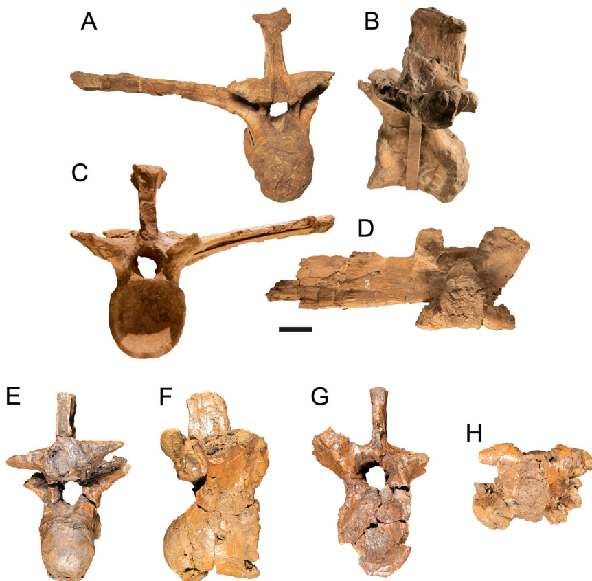
FIGURE 2. Deinosuchus hatcheri holotype specimen (CM 963) vertebrae. A–D, dorsal vertebra in A, posterior, B, lateral, C, anterior, and D, dorsal views. E–H, dorsal vertebra in E, posterior, F, lateral, G, anterior, and H, dorsal views. Scale bar equals 5 cm.
