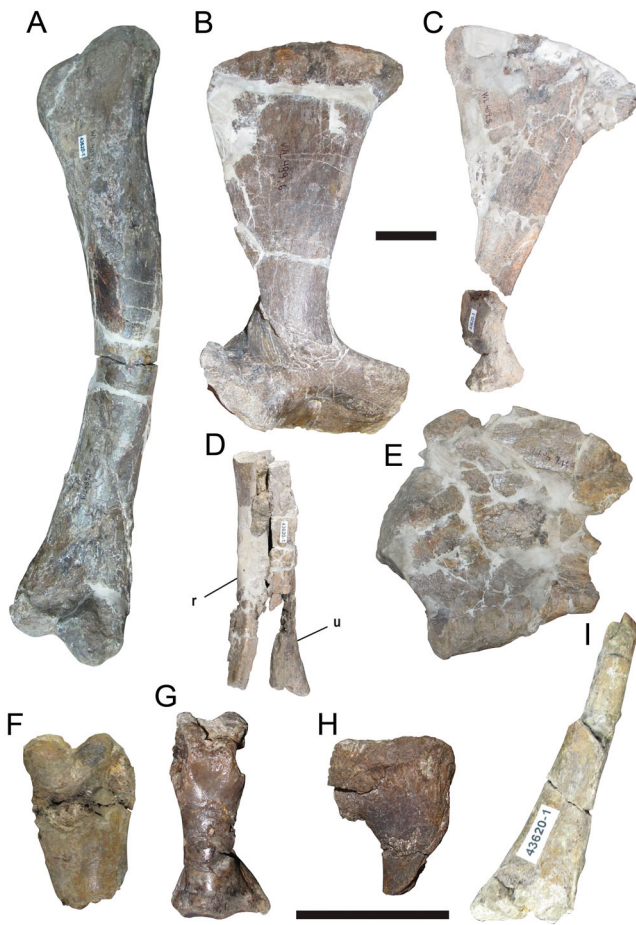
FIGURE 18. Deinosuchus riograndensis (TMM 43620-1) selected postcrania. A , right humerus in posterior view. B , left coracoid in lateral view. C , left pubis in medial view. D , left radius and ulna in posterior view. E , fragment of an ilium. F , distal end of a metapodial in anterior view. G , phalanx in anterior view. H , right proximal radiale. I , second cervical rib. Abbreviations: r, radius; u, ulna. Scale bars equal 5 cm. Top scale bar corresponds to A–E ; bottom scale bar corresponds to F–I .
