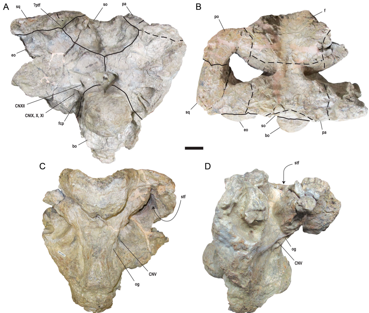
FIGURE 15. Deinosuchus riograndensis (TMM 43632-1) posterior skull. A , posterior view. B , dorsal view. C , anterior view. D , lateral view. Abbreviations: bo, basioccipital; CNV, cranial nerve V; CNIX, cranial nerve IX; CNX, cranial nerve X; CNXI, cranial nerve XI; CNXII, cranial nerve XII; eo, exoccipital; f, frontal; fcp, foramen caroticum posterius; fm, foramen magnum; og, ophthalmic groove; pa, parietal; po, postorbital; ptf, posttemporal fenestra; so, supraoccipital; sq, squamosal; stf, supratemporal fenestra. Scale bar equals 5 cm.
