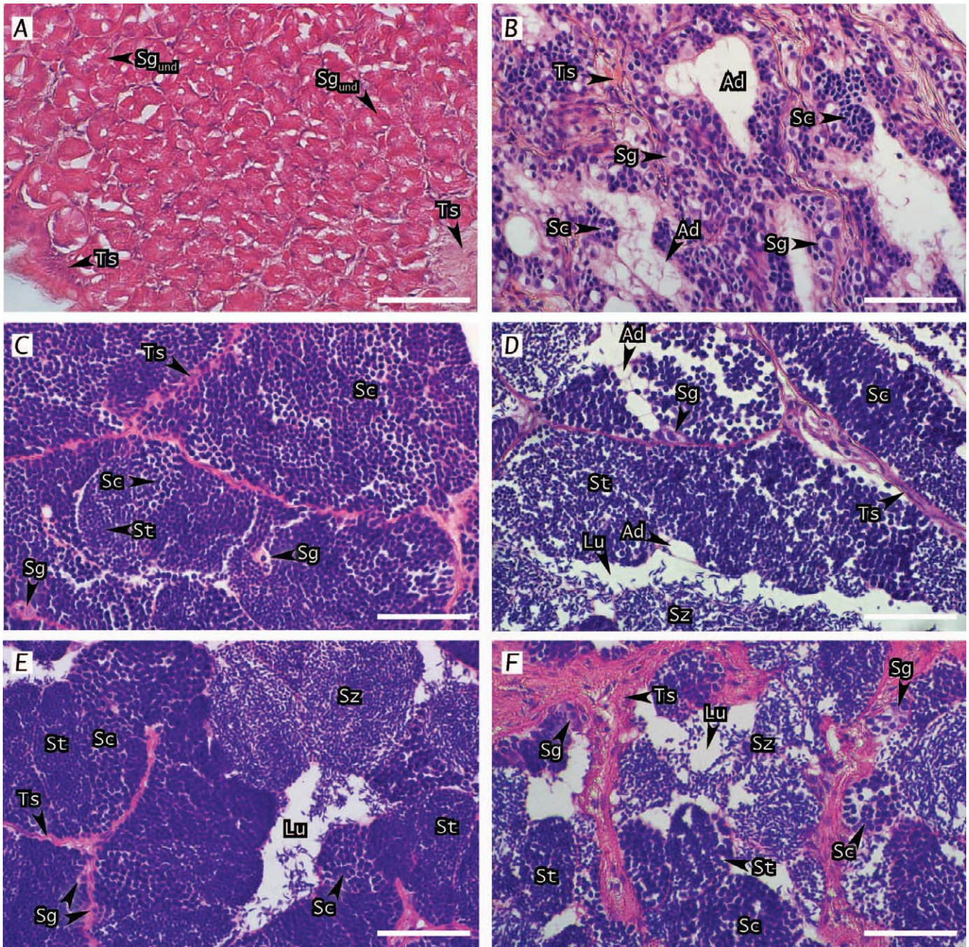
FIGURE 4. Photomicrographs (scale bar = 50 \mu m).of histological sections, illustrating characteristics of European eel testes at different stages of development during hormonally induced spermatogenesis: (A) sample week 0 ( Sg_{und} = undifferentiated spermatogonia; Ts = testicular somatic cells), (B) week 2 (Sg = differentiated spermatogonia of types A and B; Sc = spermatocytes; Ad = adipocytes), (C) week 4 (St = spermatids), (D) week 7 (Sz = spermatozoa; Lu = lumen), (E) week 12, and (F) week 18.
