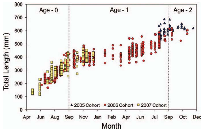
FIGURE 1. Total length versus date of capture for the three red drum cohorts that were encountered during 2007–2009 sampling in the New River estuary, North Carolina. Dashed vertical lines denote the biological birthdate of 1 September. Daily ration estimation was completed during the May–October period of rapid growth.
