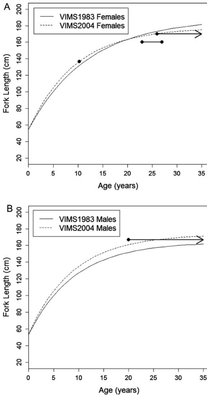
FIGURE 5. Comparison of the results of the VB3 growth model when fitted to the VIMS1983 and VIMS2004 data sets for (A) female and (B) male Sandbar Sharks. The circles represent the lower and upper estimates of bomb-radiocarbon-validated age-length data for Sandbar Sharks from the WNA (Andrews et al. 2011). A single circle signifies that a single age was given for that sample. Two circles connected with a bar represent the range for a single sample. An arrow signifies that no upper estimate was given.
