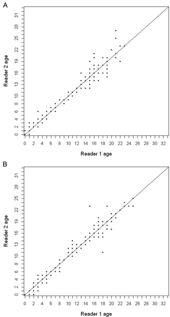
FIGURE 2. Age bias plots for readers 1 and 2 for the VIMS1983 (upper panel) and VIMS2004 (lower panel) data sets. In each panel the solid line has slope of 1 and an intercept of 0, representing no bias between readers.
