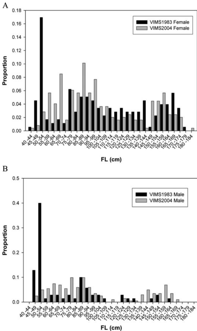
FIGURE 1. Length frequencies of (A) female and (B) male Sandbar Sharks from the VIMS1983 and VIMS2004 data sets.
