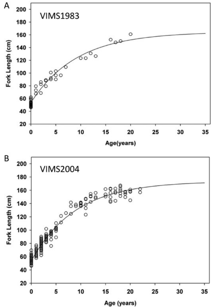
FIGURE 4. VB3 model fits and length-at-age data for male Sandbar Sharks from the (A) VIMS1983 and (B) VIMS2004 data sets.
