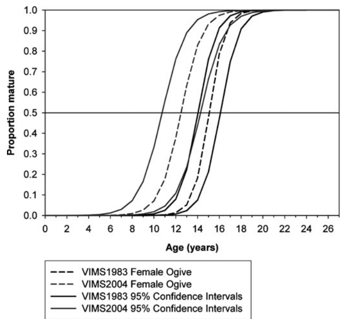
FIGURE 6. Ogives fitted to Sandbar Shark female maturity data for the VIMS1983 and VIMS2004 data sets using maximum likelihood estimation.
