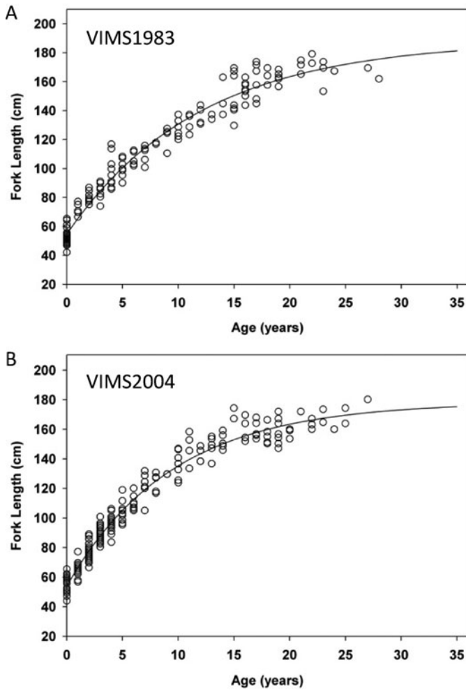
FIGURE 3. VB3 model fits and length-at-age data for female Sandbar Sharks from the (A) VIMS1983 and (B) VIMS2004 data sets.
