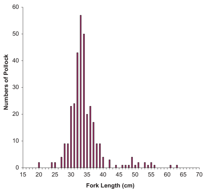
FIGURE 2. Length frequency distribution of Walleye Pollock that were used in the tagging feasibility study.
