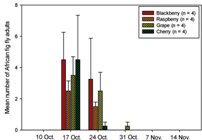
Fig. 2. Mean seasonal weekly adult captures of Zaprionus indianus , African fig fly, in ACV traps in various fruit crops (blackberry, raspberry, grape, and cherry) in Adams County, Pennsylvania, during 2012. Each bar represents standard error of mean.
