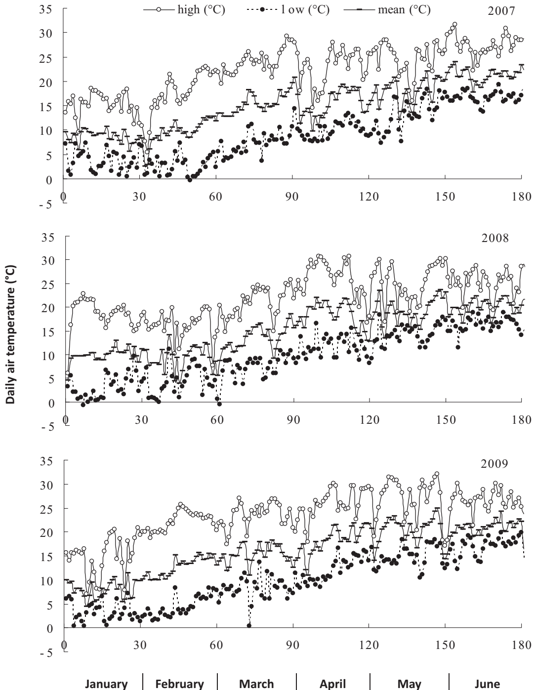
Fig. 2. Maximum, minimum, and mean daily air temperatures from 1 January through 30 June in 2007–2009 in Anning County (24.97°N, 102.33°E, 1800 m a.s.l) that were recorded at an official weather station about 8 km from our study site.
