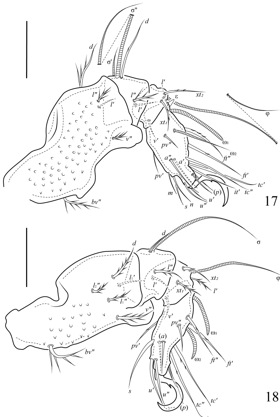
FIGURES 17–18. Papillacarus (Vepracarus) hexagonus sp. nov. , adult: legs, femur to tarsus, antiaxial view. 17. leg I, right; 18. leg II, right; Scale bar 50 \mu m.
