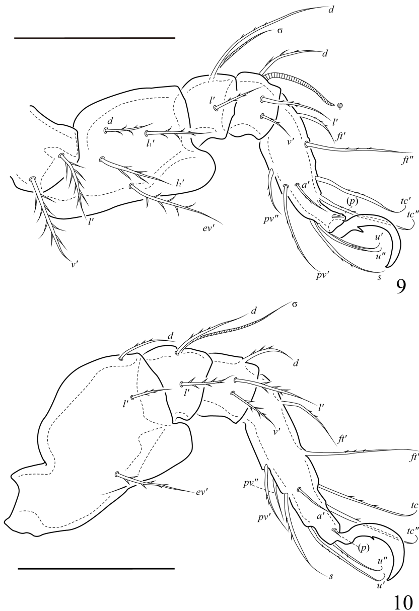
FIGURES 9–10. Papillacarus (Papillacarus) internus sp. nov., adult: legs, femur to tarsus, antiaxial view. 9. leg III, left; 10. leg IV, left. Scale bar 50 \mu\text{m} .
