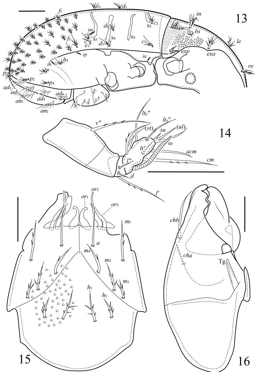
FIGURES 13–16. Papillacarus (Vepracarus) hexagonus sp. nov. , adult: 13. lateral view; 14. palp, right; 15. subcapitulum, ventral view; 16. chelicera, left. Scale bar 50 \mu m (13), 25 \mu m (14, 15, 16).
