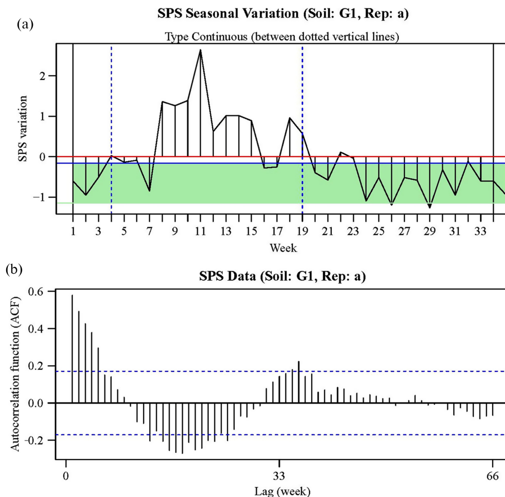
Fig. 5. Time series showing a seasonal pattern of soil phosphorus saturation (SPS) variation (a; upper figure) over a 33 wk cycle per year, followed by the autocorrelation function (b; lower figure) of SPS (correlation versus lag). [Colour online.]
