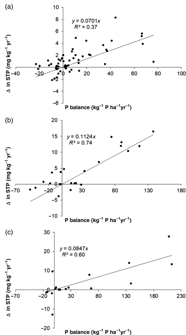
Fig. 2. Linear relationships derived from the literature showing the change in soil test phosphorus (STP) concentrations ( \text{mg kg}^{-1} \text{yr}^{-1} ) for (a) Olsen, (b) Mehlich 3, and (c) modified Kelowna STP as affected by the mean annual P balance ( \text{kg P ha}^{-1} \text{yr}^{-1} ).
