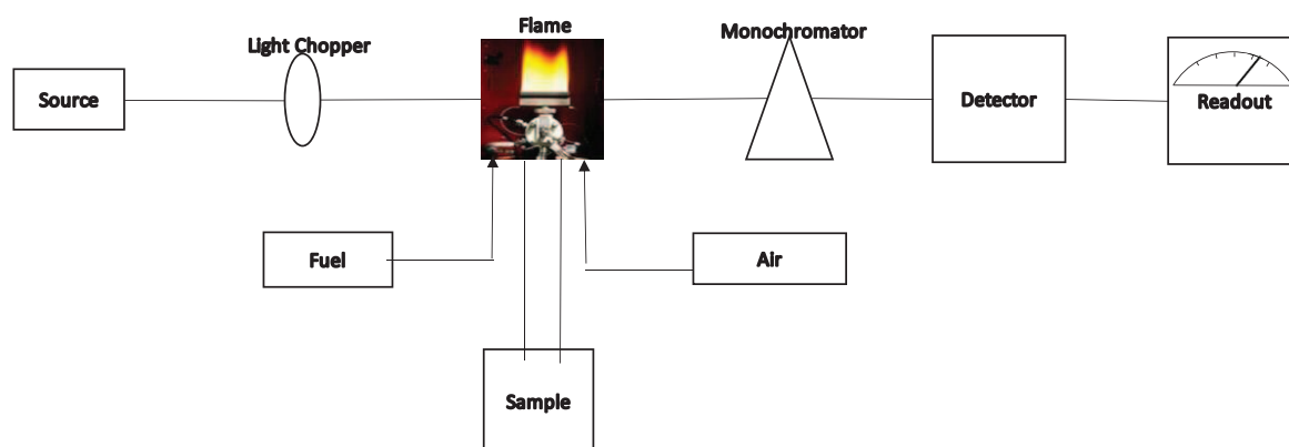
Plate 2. A typical layout of a flame AAS.
