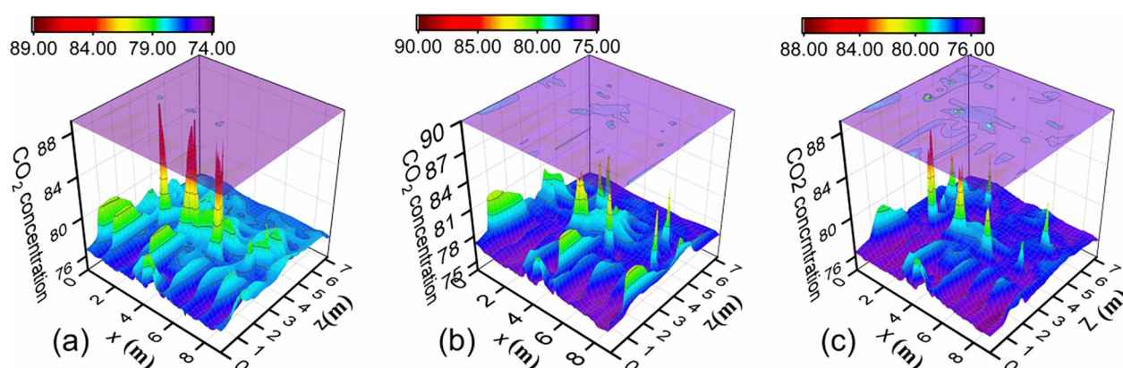
Figure 13. Three-dimensional surface diagram of the breathing zone CO 2 concentration at the 3 outlet positions under evaporative cooling air conditioning, (a–c) represent outlet-a, outlet-b, outlet-c, respectively.
