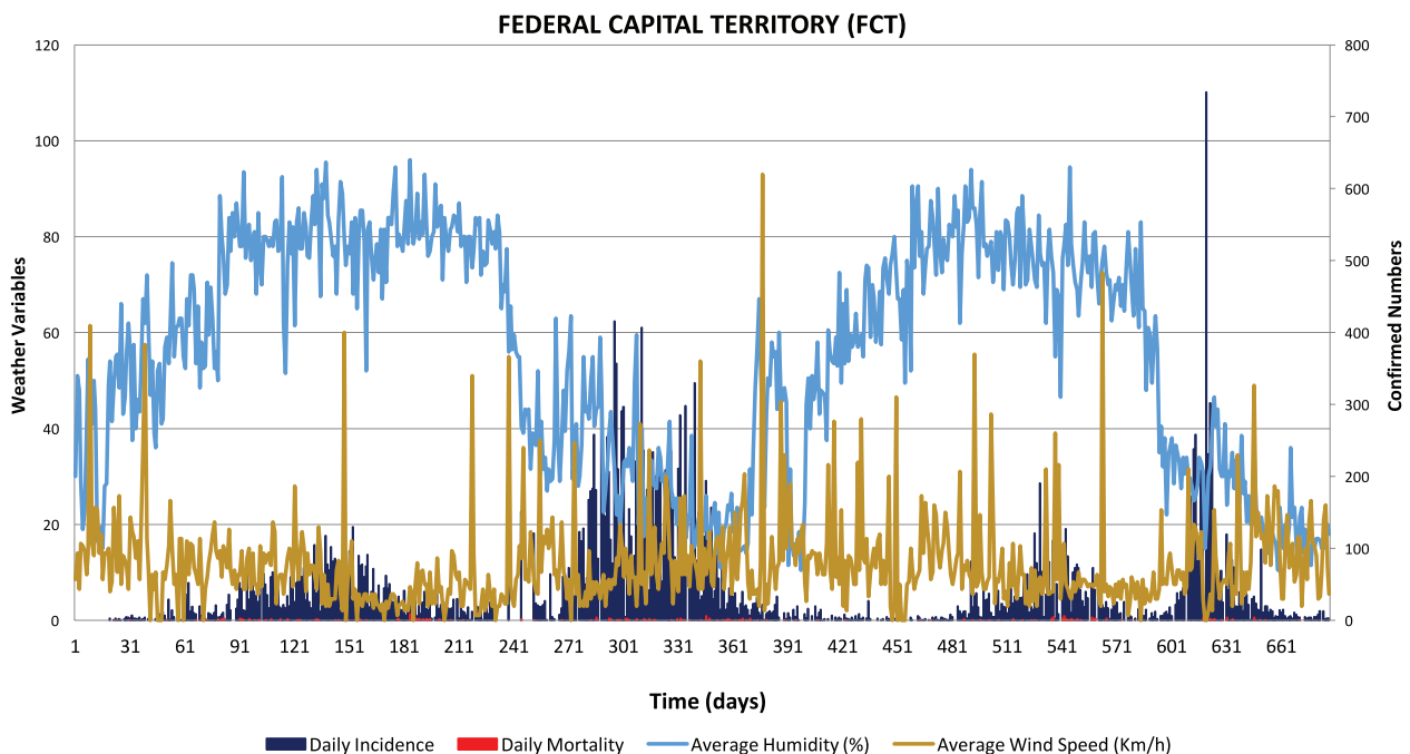
Figure 2. A time series plot showing the relationship between weather variables and incidence/mortality due to COVID-19 in the Federal Capital Territory (FCT), Nigeria between March 2020 and February 2022.
