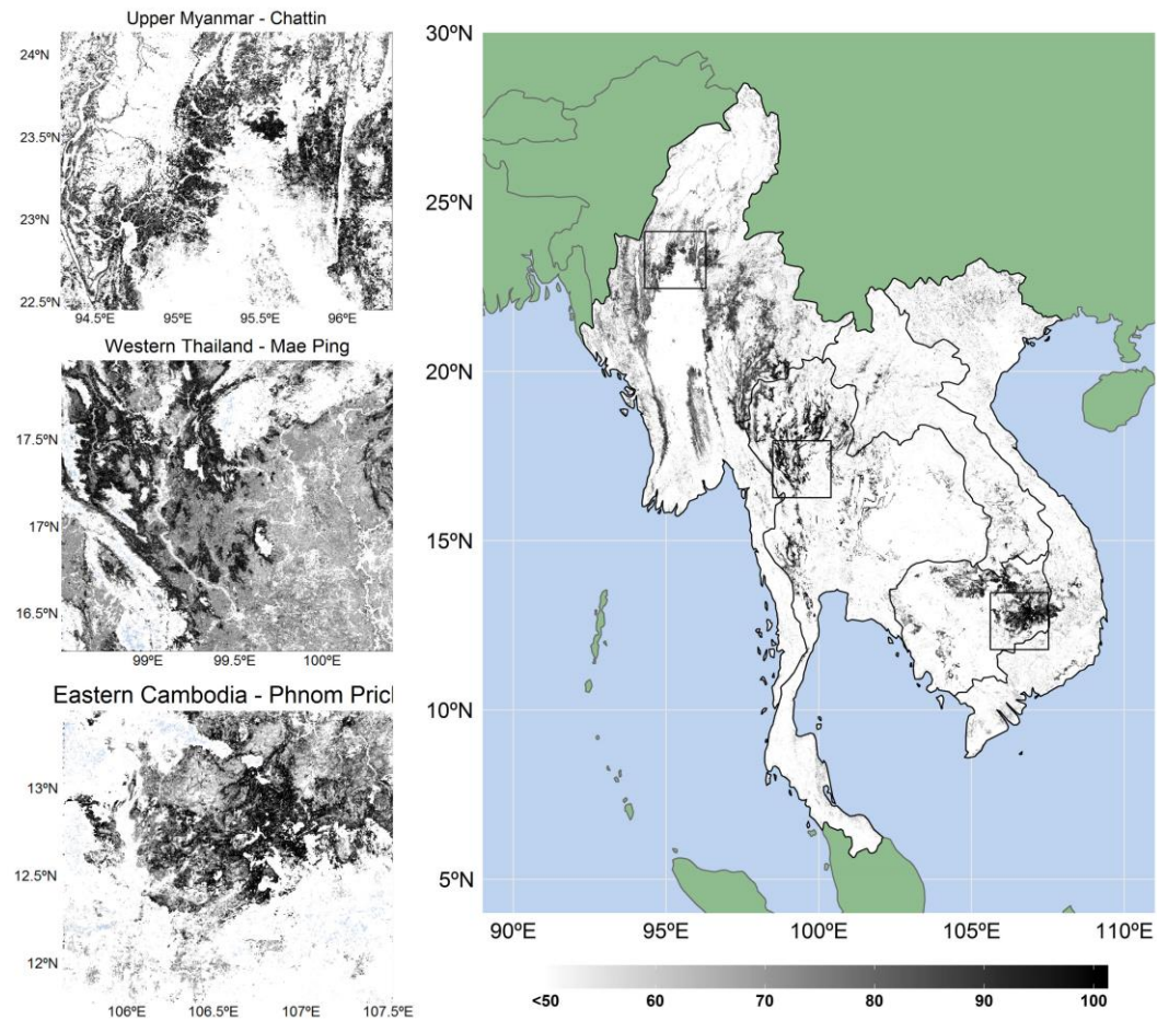
Fig 5. Spatial distribution of dry deciduous dipterocarp forest coverage (in %) in South-east Asia and the three geographical subregions in upper Myanmar, western Thailand, and eastern Cambodia in 2011.
