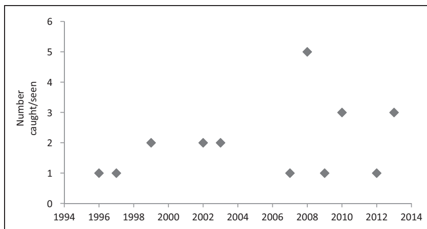
Figure 4. Number of Saola observations per year based on this study. The highest number of Saola records coincide to when roads started to be constructed through the area in 2008. The most recent sightings were in 2013 (three sightings) in and around Phou Sithon Endangered Species Conservation Area.
