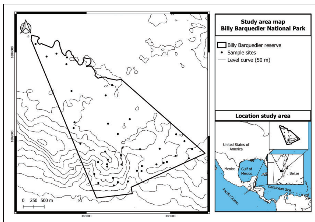
Figure 1. Location and Samples Sites at the Billy Barquedier National Park, Stann Creek Valley District, Southeast Belize (17°02′24.3″–88°27′32.0″ N, 17°01′50.0″–88°26′20.6″ W).
