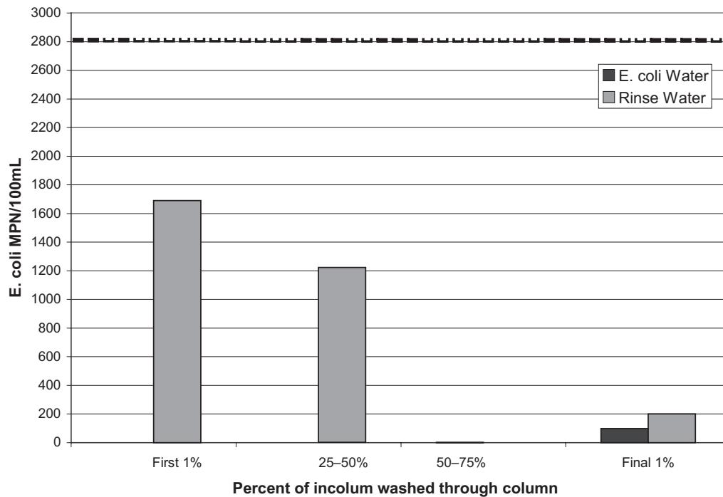
Figure 3. E. coli MPN/100mL from various portion of the effluent a 15 cm test column and 1.5:1 (Biofilter mix:sand) ratio. Starting E. coli inoculum for this trial is represented by the dashed line and was 2.83E3 E. coli /100mL.
