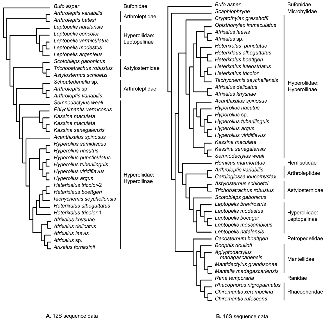
Fig. 28. Maximum-likelihood tree of hyperoliid, arthroleptid, and astylosternid frogs provided by Vences et al. (2003c). A , Maximum-likelihood analysis of 12S rRNA molecule (187 informative sites) analyzed under a GTR substitution model (cost functions reported) suggested by Modeltest (Posada and Crandall, 1998). Initial alignments under Clustal software, costs not disclosed, and subsequently adjusted manually. Highly variable regions and gaps were excluded as evidence. B , Maximum-likelihood trees based on 138 informative sites of 16S rRNA molecule under a GTR substitution model (cost functions reported) for hyperoliids, arthroleptids, and astylosternids. Initial alignments were made under Clustal, costs not disclosed, and subsequently adjusted manually. Highly variable regions and gaps sites were excluded as evidence.
