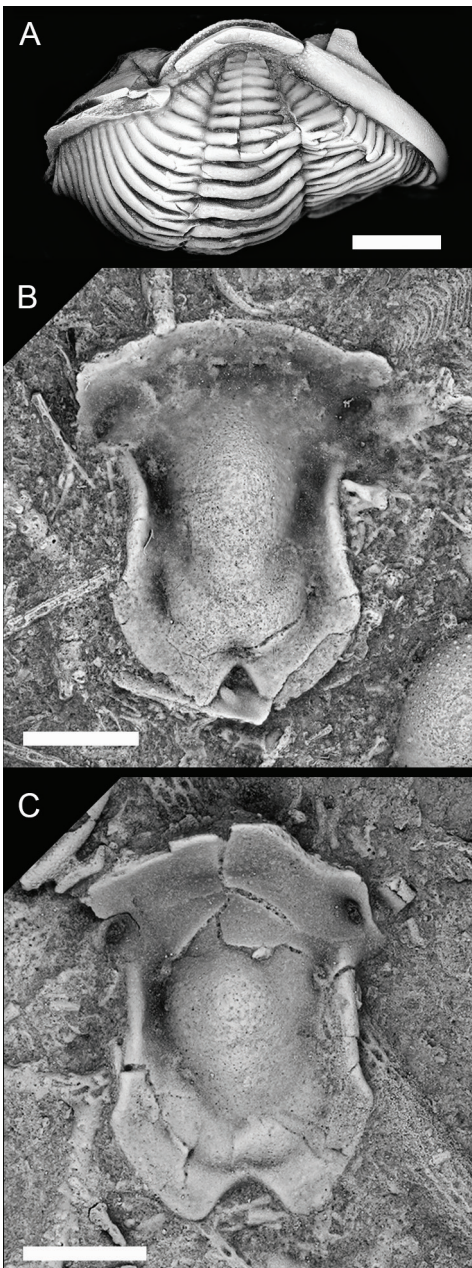
FIGURE 6. Ventral morphology of Flexicalymene trentonensis , n. sp. A. View of rostral plate, AMNH-FI-140955 (paratype), scale bar = 5 mm. B. ?Hypostome, MCZ 201041, scale bar = 2 mm. C. ?Hypostome, MCZ 201403, scale bar = 2 mm. MCZ specimens are from the Walcott-Rust Quarry; AMNH-FI-140955 is from the type locality in Quebec (see text).
