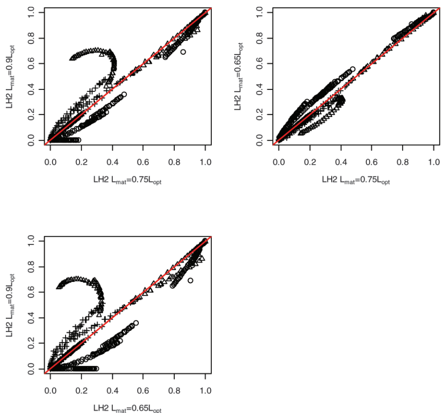
FIGURE 4.—Relationships between the catch-based length proportions (open circles = P_{\text{mat}}^{\text{mega}} ; open triangles = P_{\text{opt}} ; crosses = P_{\text{mat}} ; each defined in Methods) for different ratios of length at maturity ( L_{\text{mat}} ) to optimal fishing length ( L_{\text{opt}} ) for life history 2 (LH2; defined in Table 1) across all selectivity patterns, fishing mortality rates, and steepness values. The solid red line is a 1:1 reference line.
