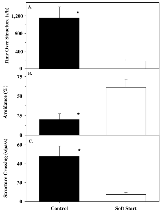
FIGURE 3.—Behaviors (mean \pm SE) of white sturgeon within the raceway for control fish and fish subjected to the soft-start pulse type: (A) time for which the fish occupied the water column above the electrical barrier system; (B) percentage of observed events in which the fish approached the electrical system, turned, and returned as opposed to passing over the system; and (C) time taken by the fish to cross the system. Asterisks indicate significant ( P < 0.05 ) differences between control and treatment fish.
