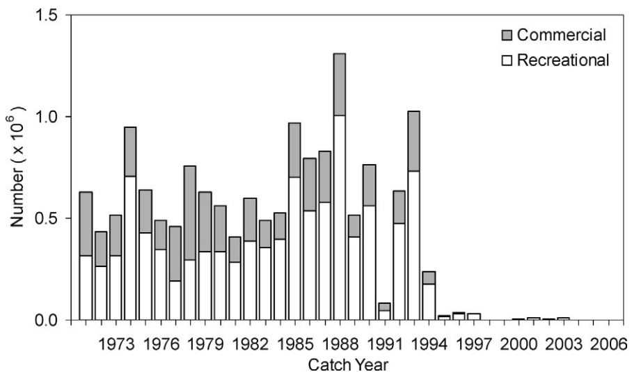
FIGURE 2.—Commercial and recreational catches (numbers of fish) of coho salmon in the Strait of Georgia (1971–2006). The catch year is the second ocean year and the year in which they would return to spawn. The ocean entry year is 1 year earlier.
