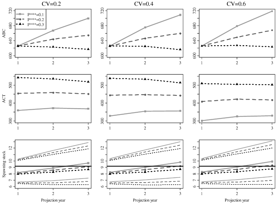
FIGURE 3.—Example of Integrated PASCL applied to vermilion snapper, with P^* = 0.4 and P^{***} = 0.1, 0.2 , or 0.3 , as indicated. The CV of management implementation was assumed to be 0.2, 0.4 , or 0.6 , as shown in the column headings. The top two rows show catch levels, ABCs, or ACTs (metric tons). The bottom row shows median spawning stock ( 10^{12} eggs) from 10,000 replicates, upper and lower quartiles, and the point estimate of spawning stock at maximum sustainable yield (heavy horizontal line).
