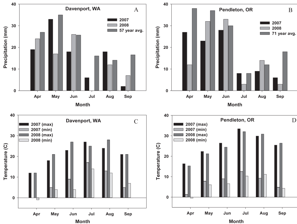
Figure 1. Mean monthly precipitation (A and B) and mean monthly maximum and minimum air temperatures (C and D) at Davenport, WA and Pendleton, OR, during study period.
