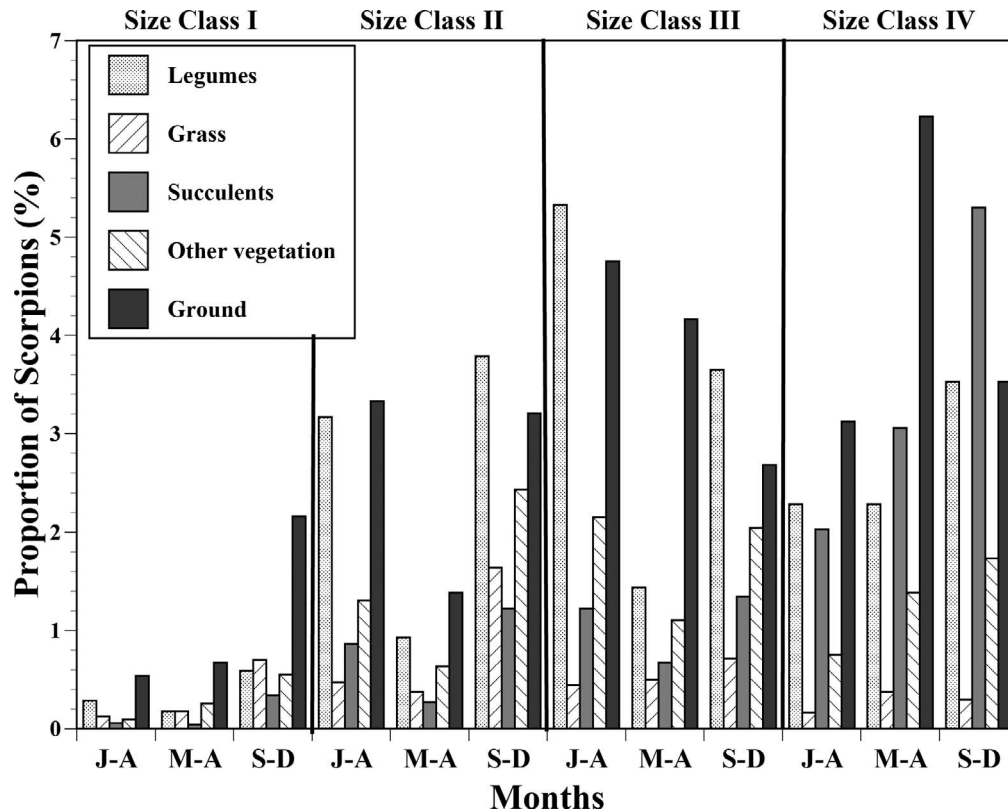
Figure 3.—The proportion (%) of C. vittatus with and without prey using different microhabitats among months of the years and scorpion size classes ( n = 7449 ). Three-way G test interaction comparison was significantly different ( G = 51.430 , df = 24 , P < 0.001 ). Months of the year were pooled with J-A = January through April, M-A = May through August and S-D = September through December. Interaction, conditional and orthogonal planned comparisons of a three-way G test of the contingency table among microhabitats, months of the year and scorpion size classes were performed but not shown. See Table 1.
