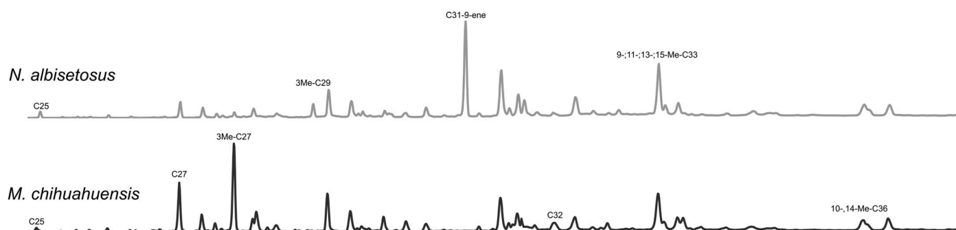
Figure 5.—Cuticular hydrocarbon (CHC) profiles of the spider Myrmecicultor chihuahuensis and Novomessor albisetosus ants. Example gas chromatographic traces of CHCs extracted from the spider and ant species. Major CHCs are labeled; complete list by retention index can be found in Table 1.
