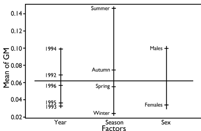
Fig. 2. Graph of interaction among years, seasons, and sex on growth in mass of Siren intermedia as calculated by increase in g per day. See Table 3 for statistics.
