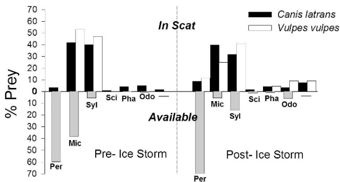
FIG. 2.—Pre- and post-ice storm comparison of number of prey consumed by Canis latrans and Vulpes vulpes relative to prey available. Prey abbreviations: Per = Peromyscus ; Mic = Microtus ; Syl = Sylvilagus ; Sci = Sciuridae ; Pha = Phasianus ; Odo = Odocoileus ; — = other vertebrates (data not available for abundance of latter food category).
